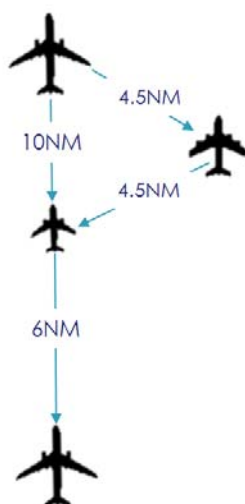
Figure 3.2.8-1 Minimum Separation
