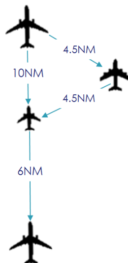
Figure 3.2.8-1 Minimum Separation
