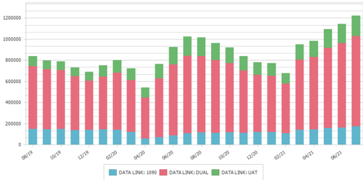
Figure 6 – Aircraft ADS-B In operations by ADS-B Link Type (1090ES, UAT, or DUAL)
