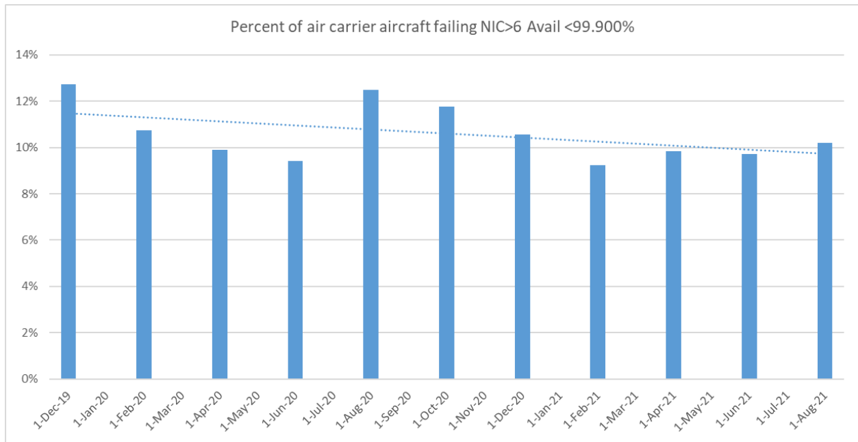
Figure 2 – Percentage of air carrier aircraft not meeting NIC>6 availability criteria
