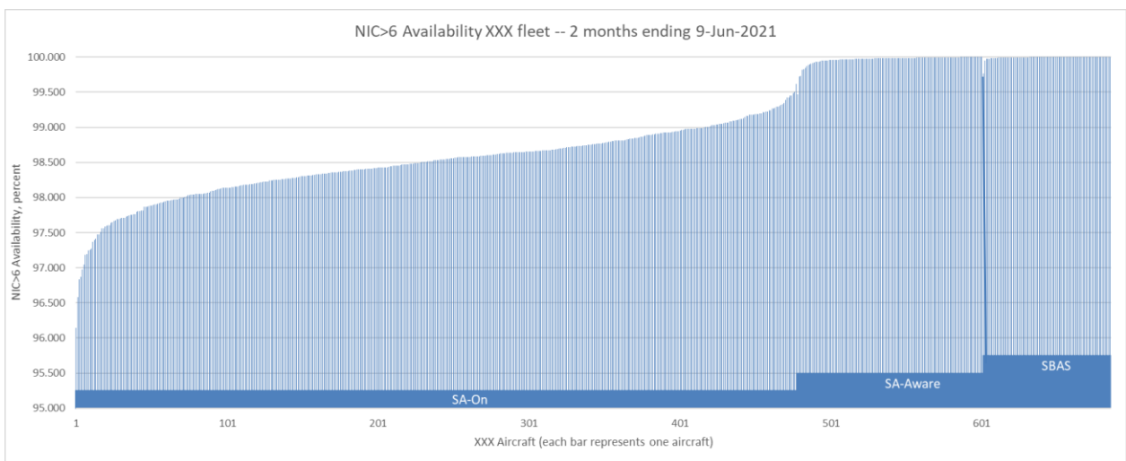
Figure 1 – NIC>6 availability performance for aircraft from XXX airline during analysis period
