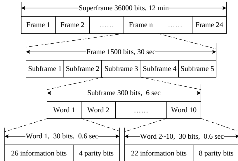
Figure B BDS-2. Frame structure of the D1 navigation message
