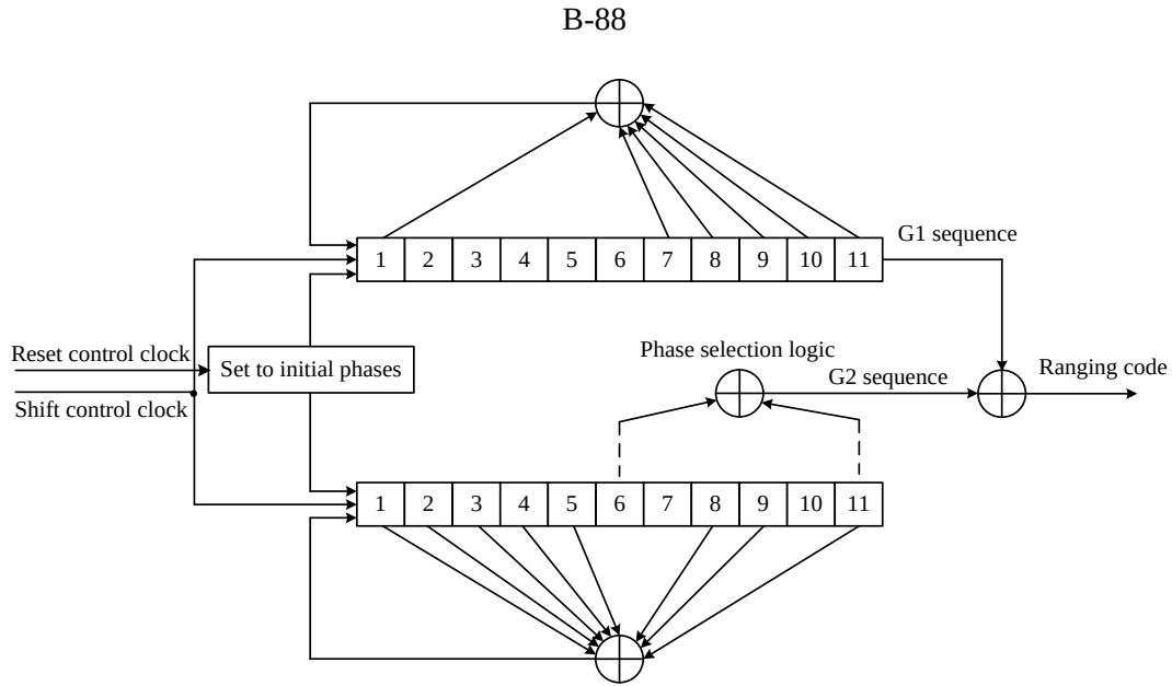
Figure B BDS-1. Generator of C_{B1I}
