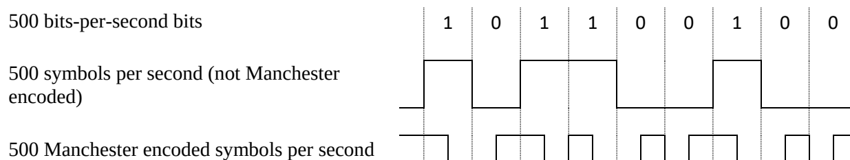
Figure D-19. Bi-binary (Manchester) encoding scheme
