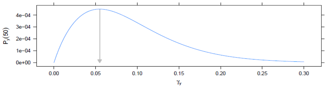
Figure 3: Wingspan overlap probability as a function of \gamma_y with S_y = 50 NM initial separation.
