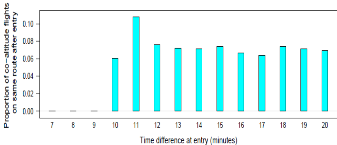
Figure 4: Values of Q(k) estimated from TSD. For co-altitude flights on the same route (after entry / before exit), the proportion of flights that entered k minutes after the preceding flight is plotted for k = 7; 8; 9; \dots; 20 minutes.
