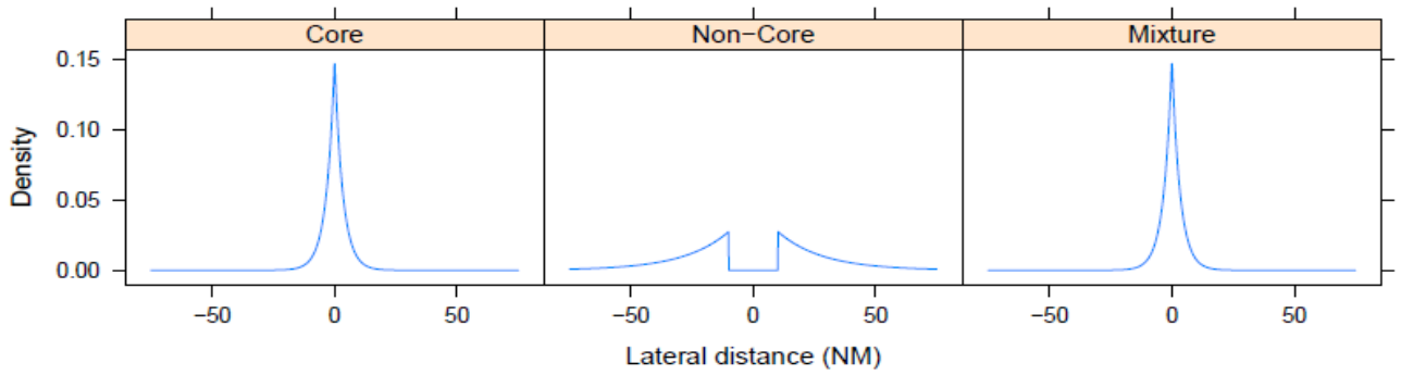
Figure 2: Modeling of lateral deviation.
