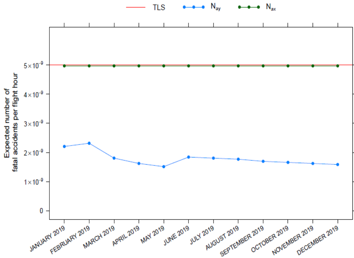
Figure 7: Assessment of Compliance with Lateral and Longitudinal TLS Values.
