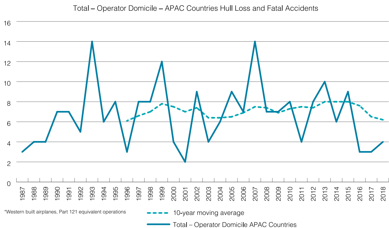
Chart 7.2.3 CAST: Number of hull loss or fatal accidents for operators based in APAC
