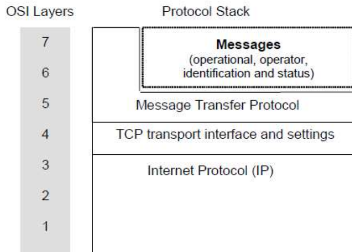
FMTM protocol stack
