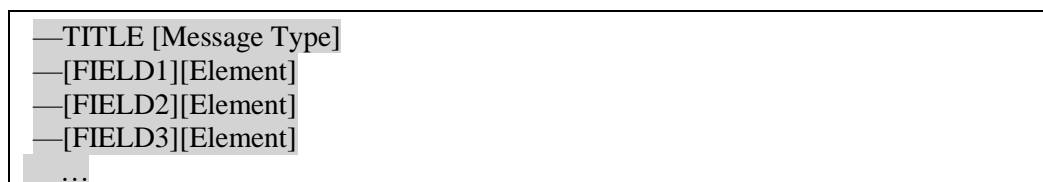
Figure 4: Overall structure of AFTN (ADEXP) message
