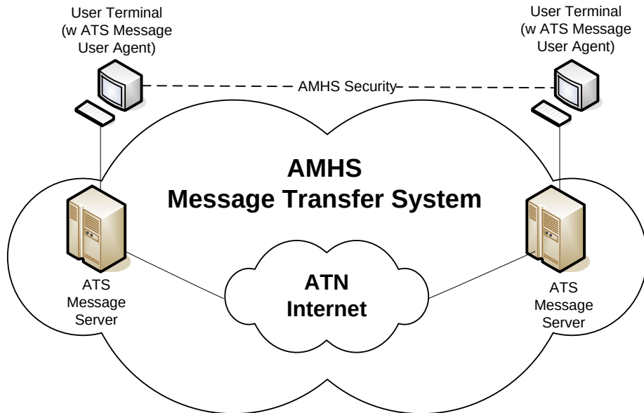
Figure 5-4: AMHS Security
