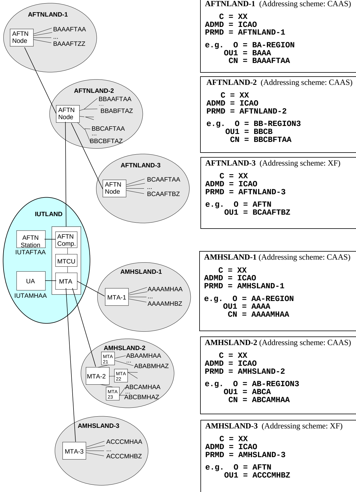
Figure 2: Addressing Plan
