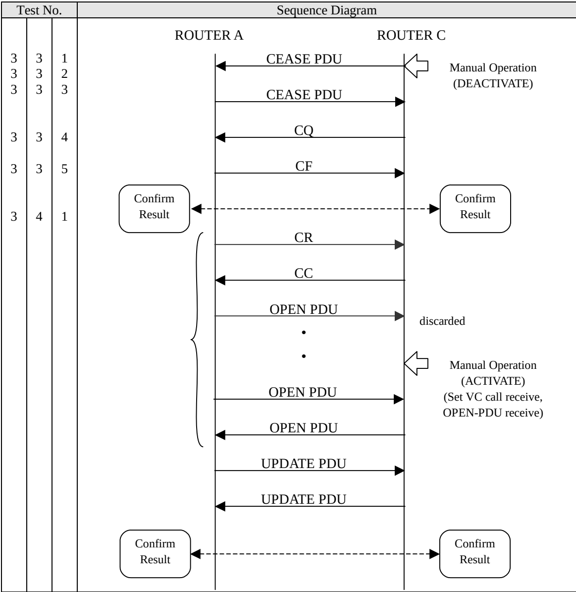
Figure 12 Sequence: Manual router Disconnection and Re-connection at AMHSLAND2 router
