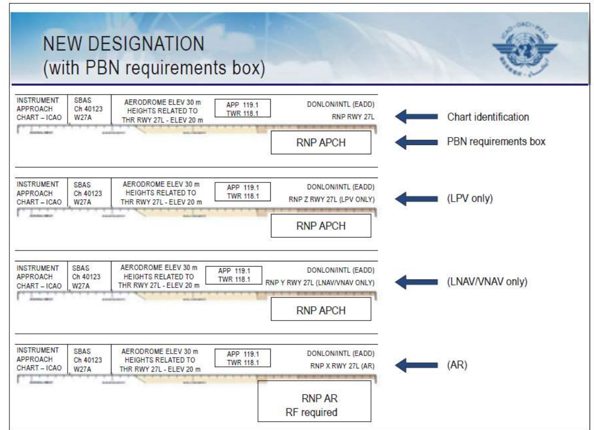
Figure 1-1. New PBN chart designation (with PBN requirements box)
