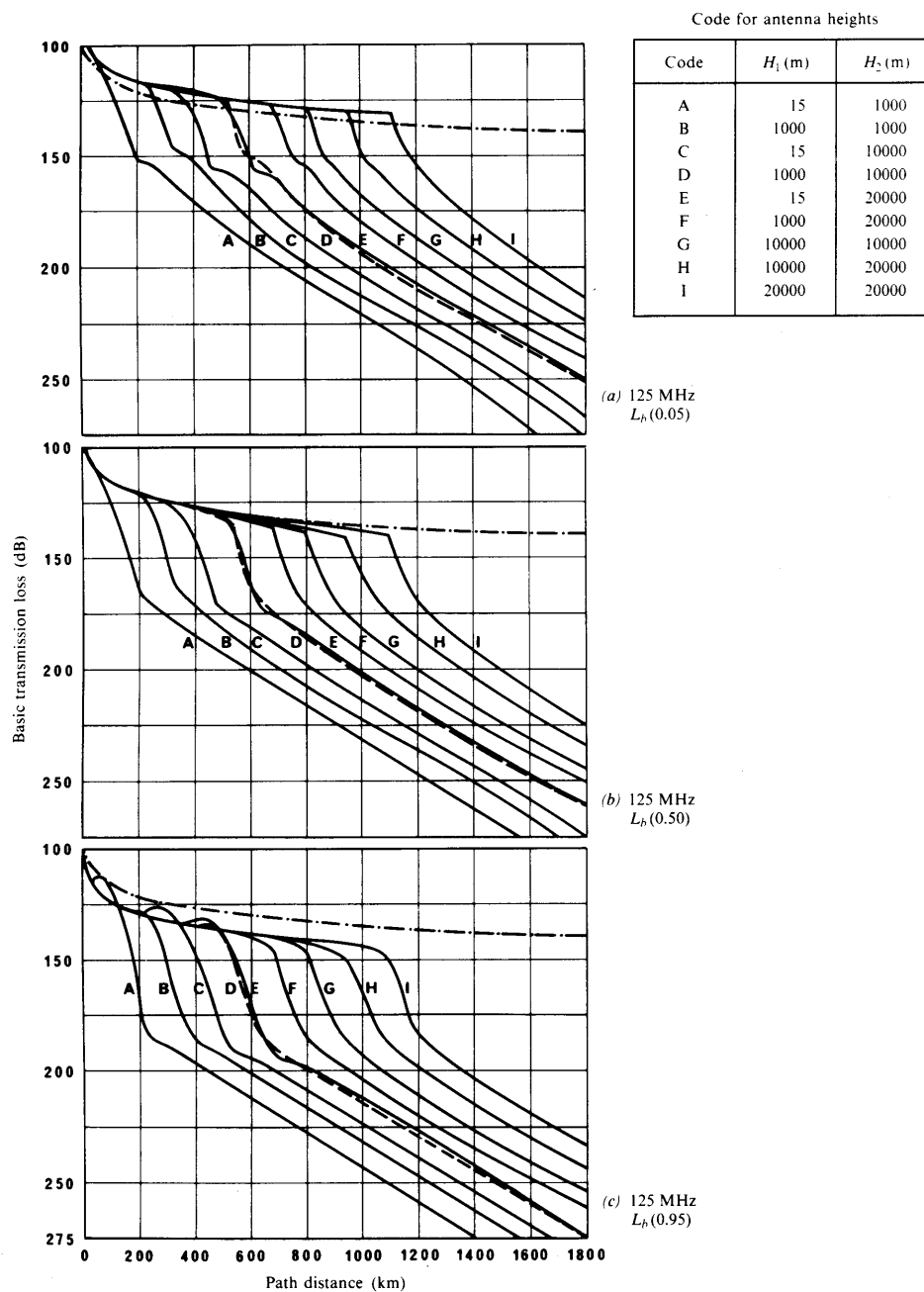
FIGURE 1 — Basic transmission loss at 125 MHz for 5%, 50% and 95% of the time
