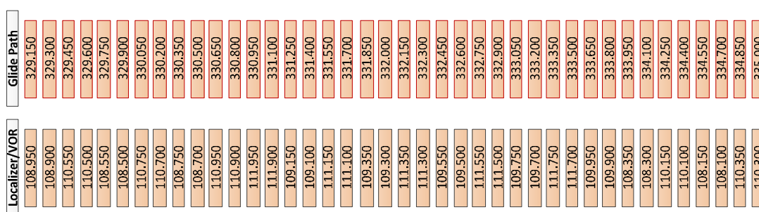
Figure 3 – 5 Overview of adjacent glide path frequencies in relation to the localizer frequency
