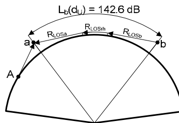
Figure 1 – 5 Separation distances (aircraft are not within line of sight)
