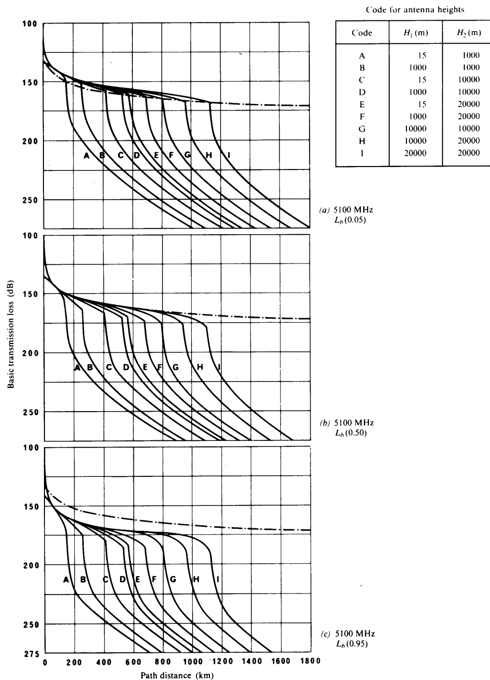
FIGURE 4 — Basic transmission loss at 5100 MHz for 5%, 50% and 95% of the time
