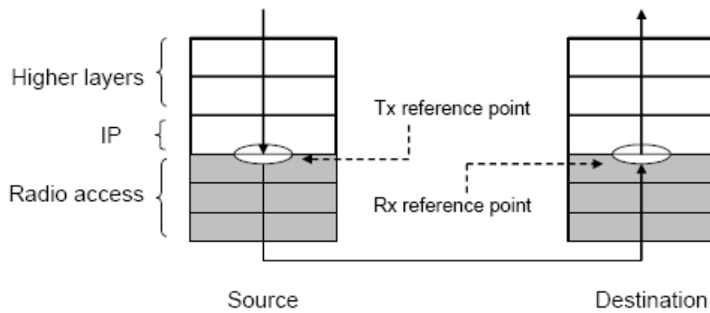
Figure 5 Illustration of reference points for the maximum data latency ( drawing reference WiMAX Forum xxx)
