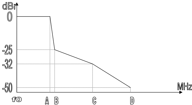
Figure 3 – Figure 3 Transmit spectral mask as provided by IEEE 802.16-2009 (8.5)
