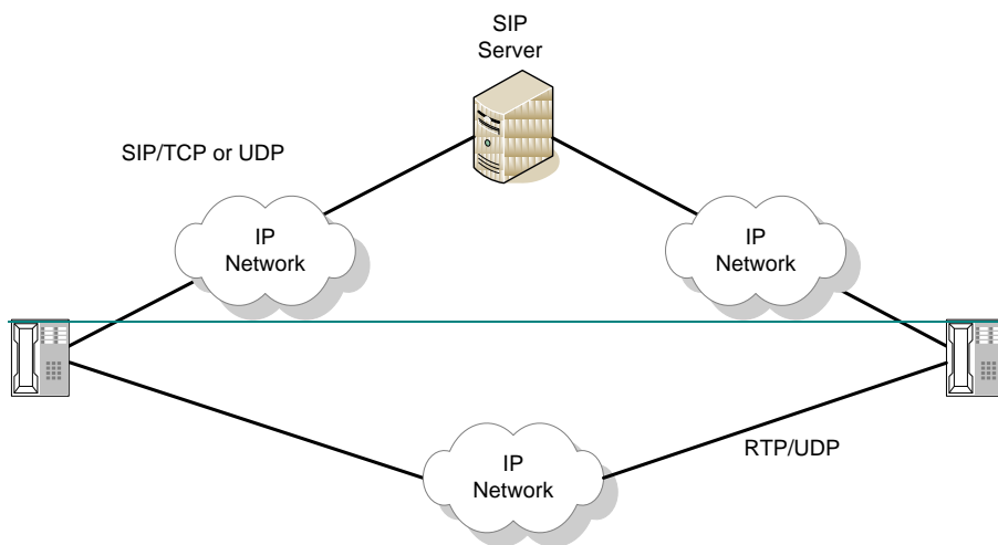
Figure 5. VoIP with SIP
