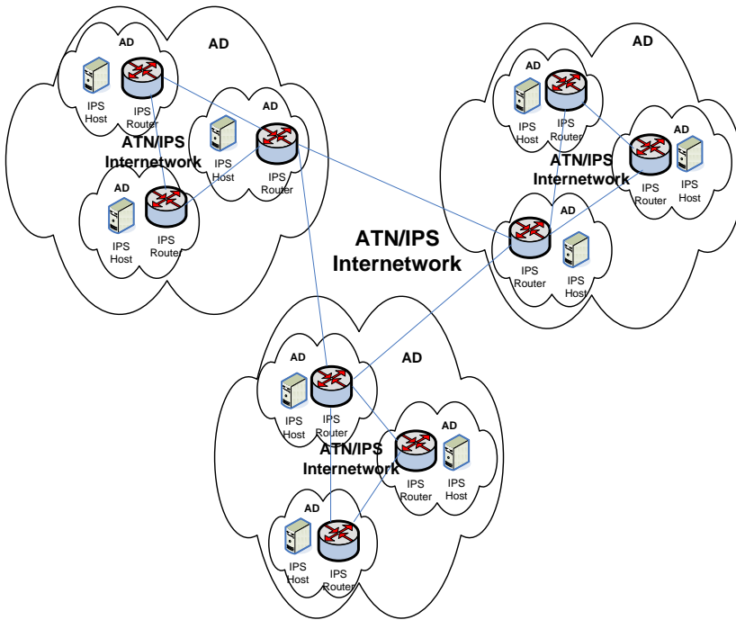
Figure 2.1-1 – The ATN/IPS Internetwork
