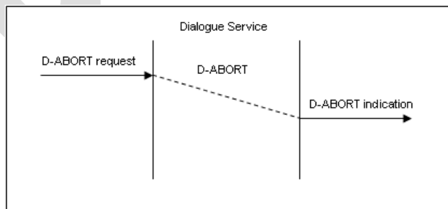
Figure 8. D-ABORT Service
