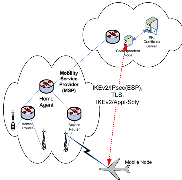
Figure 6.3.3-1 – Options for Air-Ground End-to-End Security
