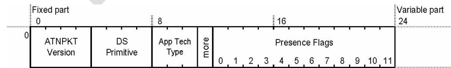
Figure 2. ATNPKT Format
