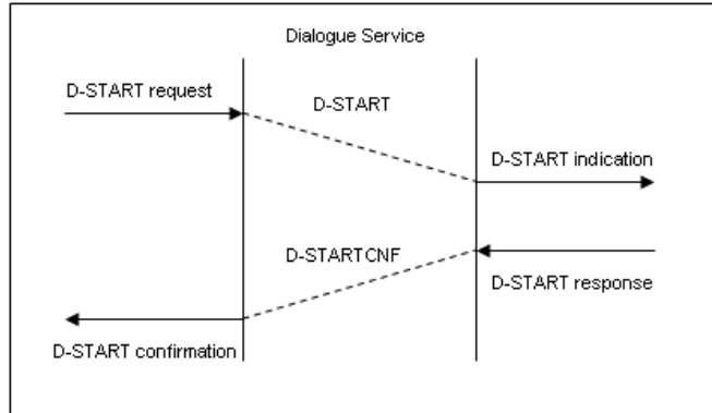
Figure 4. D-START Service
