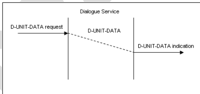
Figure 10. D-UNIT-DATA Service (TCP)
