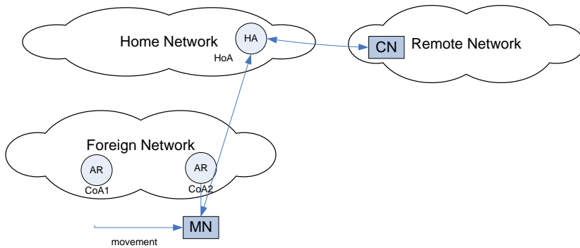
Figure 5.1-1: Mobile IP
