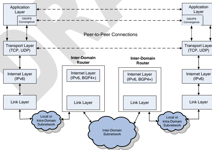
Figure 1 – ATN/IPS Protocol Architecture
