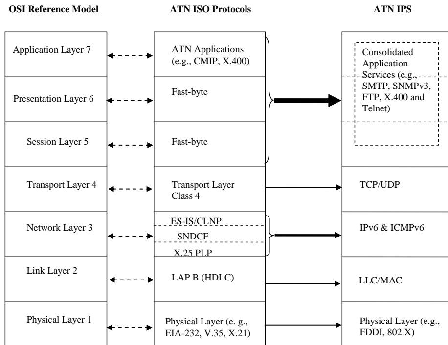
Figure 1.1 Protocol Reference Model
