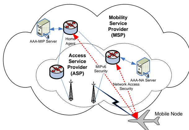
Figure 6.3.4-1 – ASP or MSP Security
