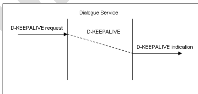
Figure 13. D-KEEPALIVE Service
