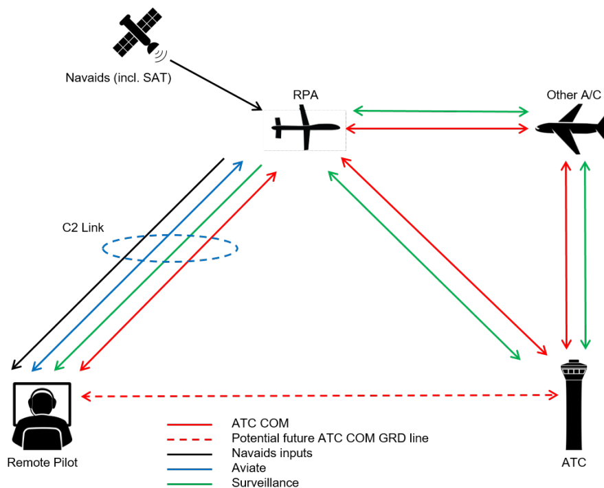
Figure 4 – System interfaces
