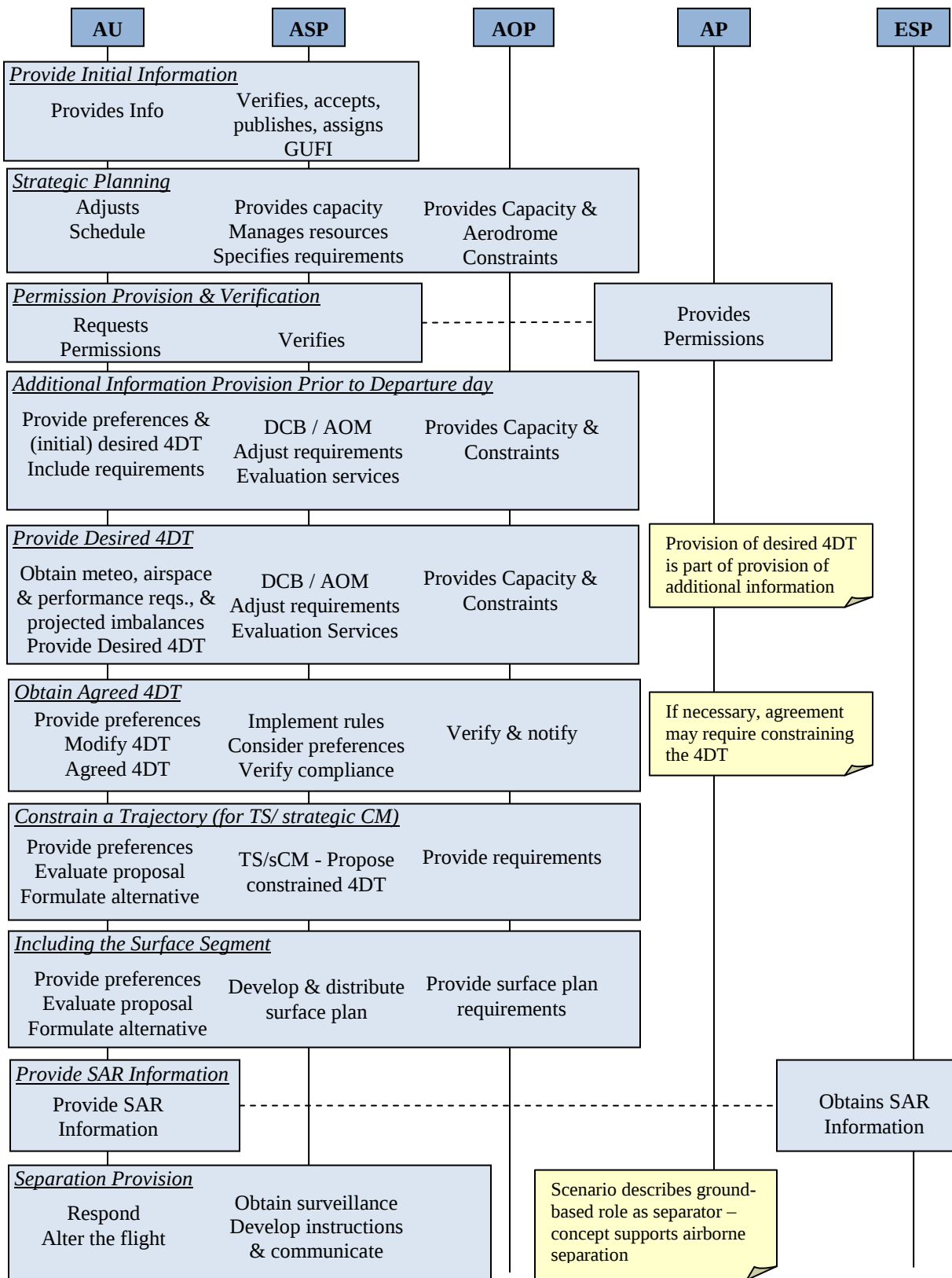
Figure 3.5-1 Role of participants in various scenarios throughout a flight's evolution
