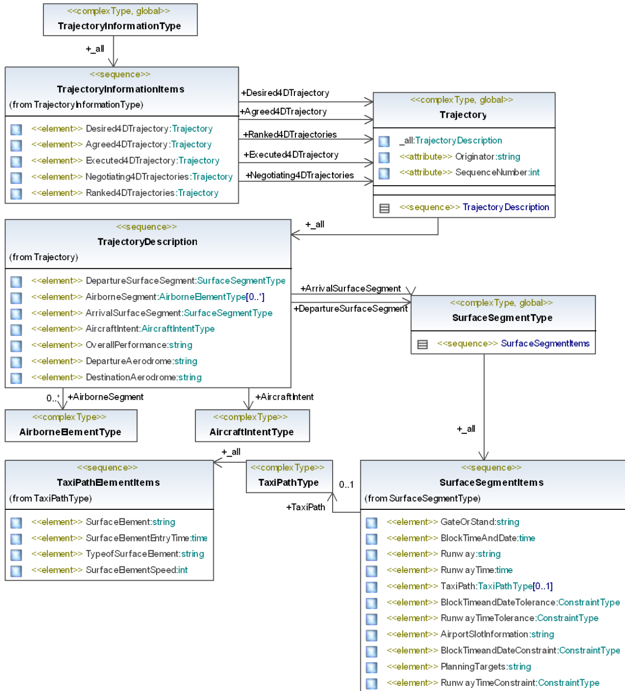
Figure G.2-10 Trajectory XML schema Diagram
