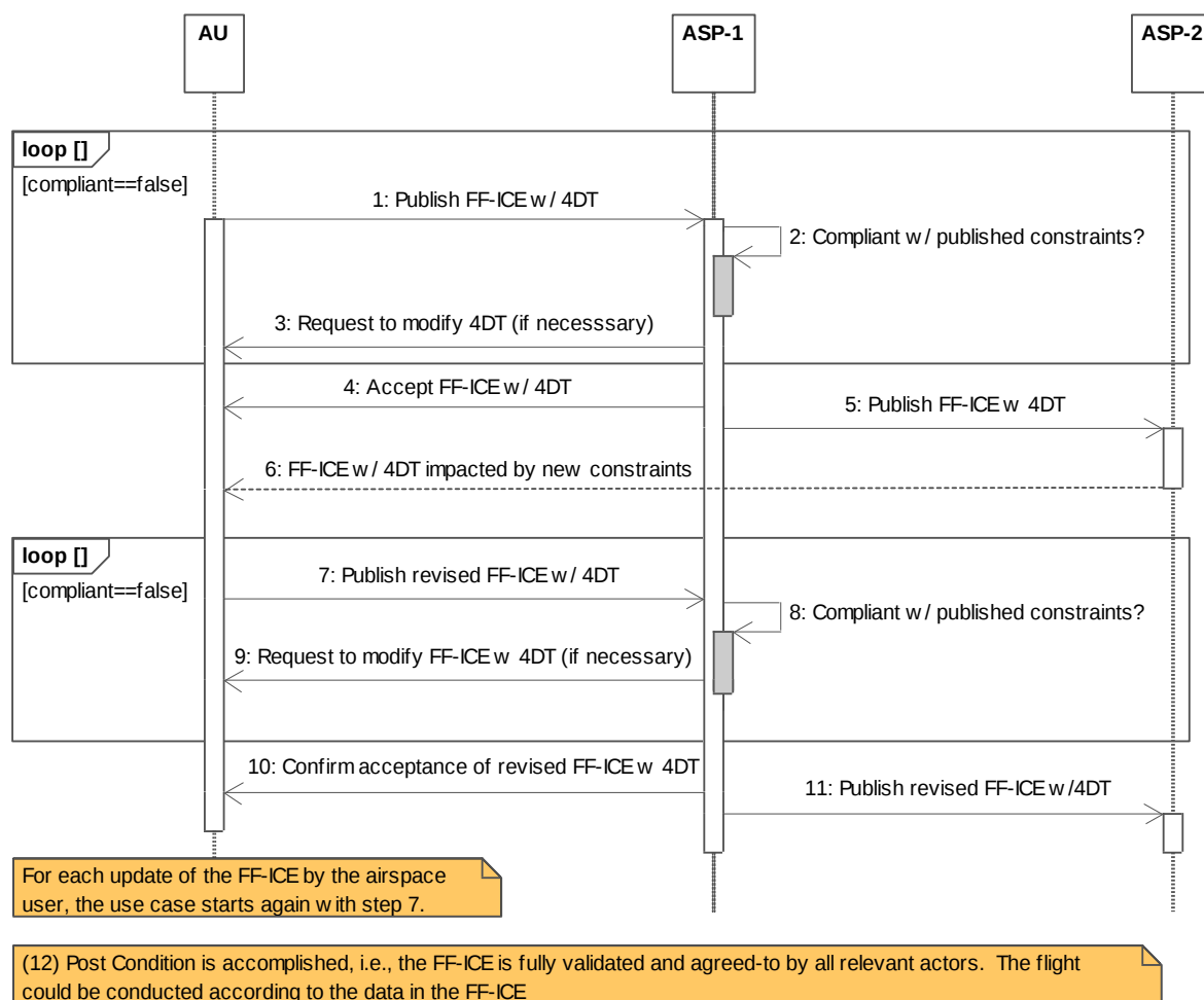
Figure C.6-3 Determining Agreed 4D trajectory using constraints (alternative approach)
