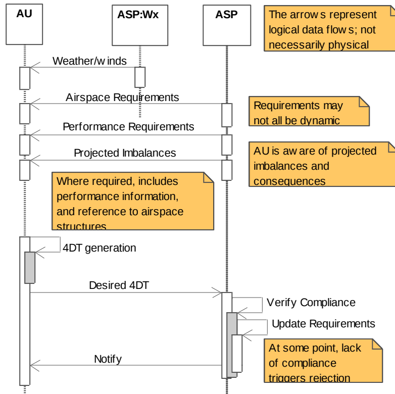
Figure C.6-1 Provision of desired 4D trajectory
