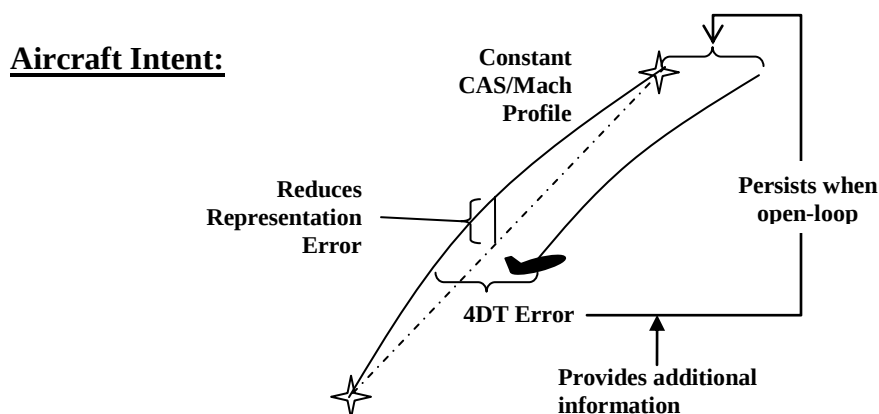
Figure D.2-2 Example of aircraft intent utility in climb
