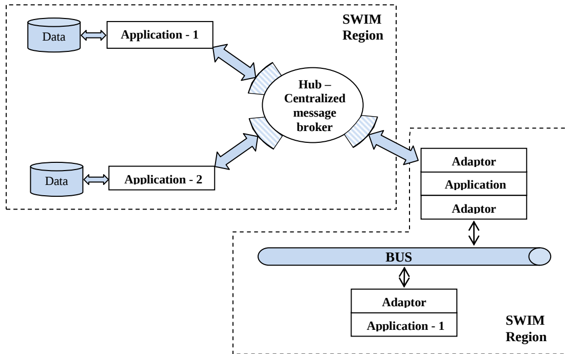
Figure H.1-7 Interface between differing SWIM Regions
