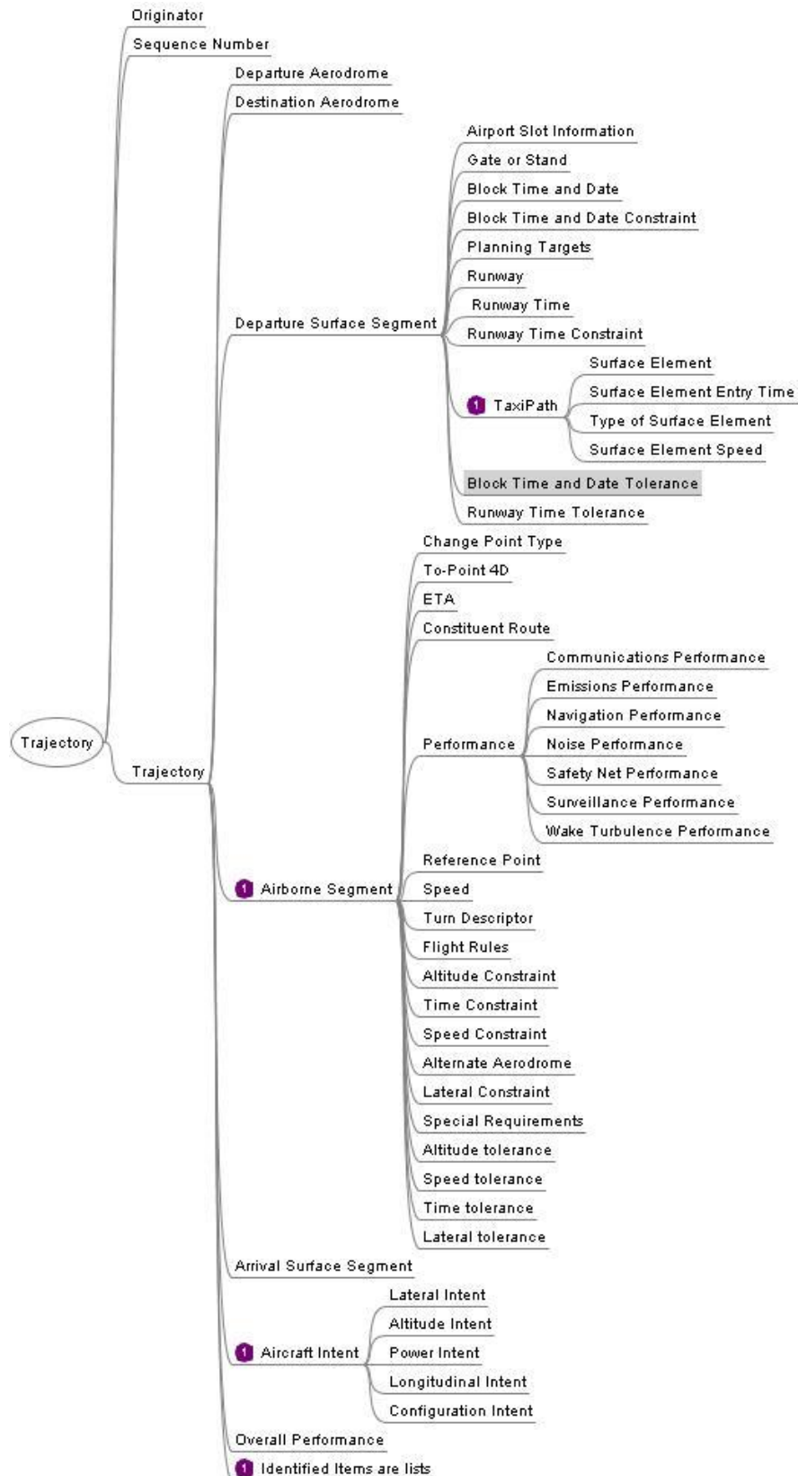
Figure G.1-2 Description of Trajectory Hierarchy
