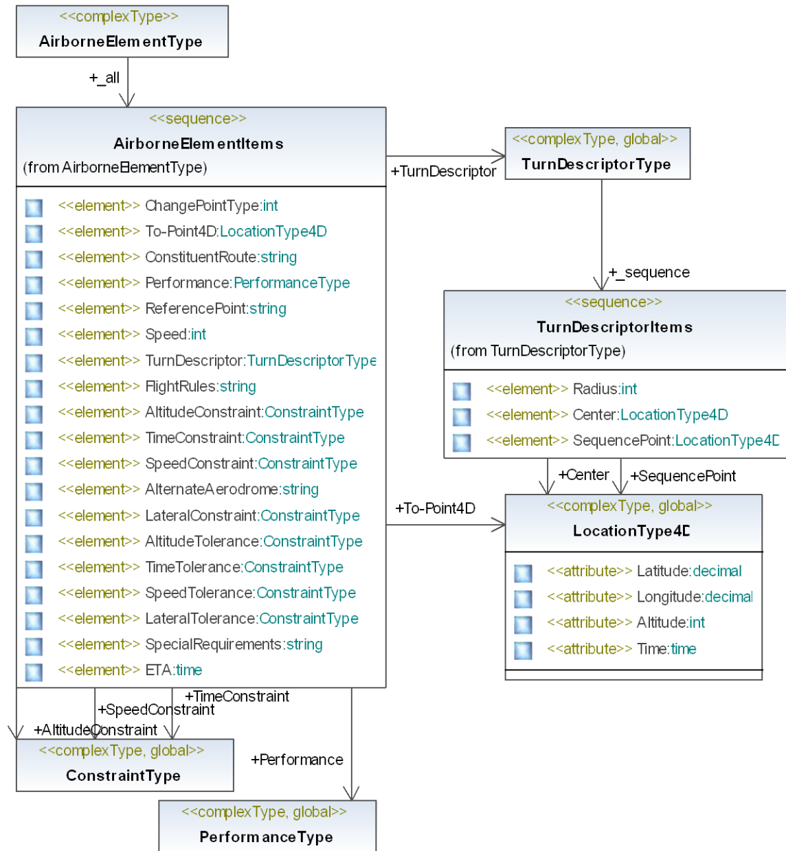
Figure G.2-2 Airborne Element XML schema Diagram
