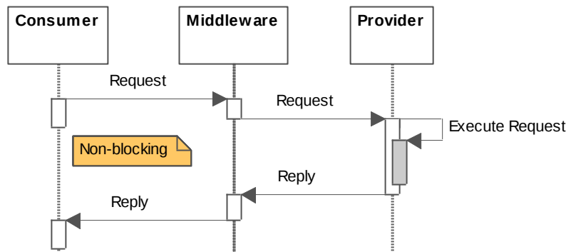
Figure H.1-6 Asynchronous request/reply message pattern
