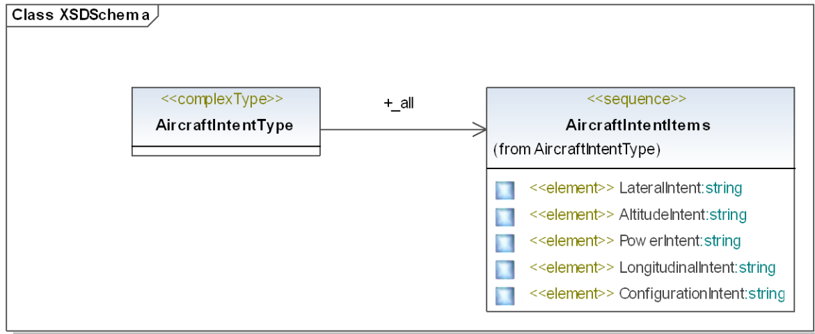
Figure G.2-3 Aircraft Intent XML schema Diagram
