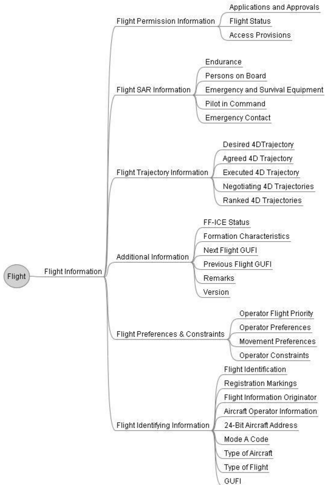
Figure G.1-1 Top-level hierarchy of information items
