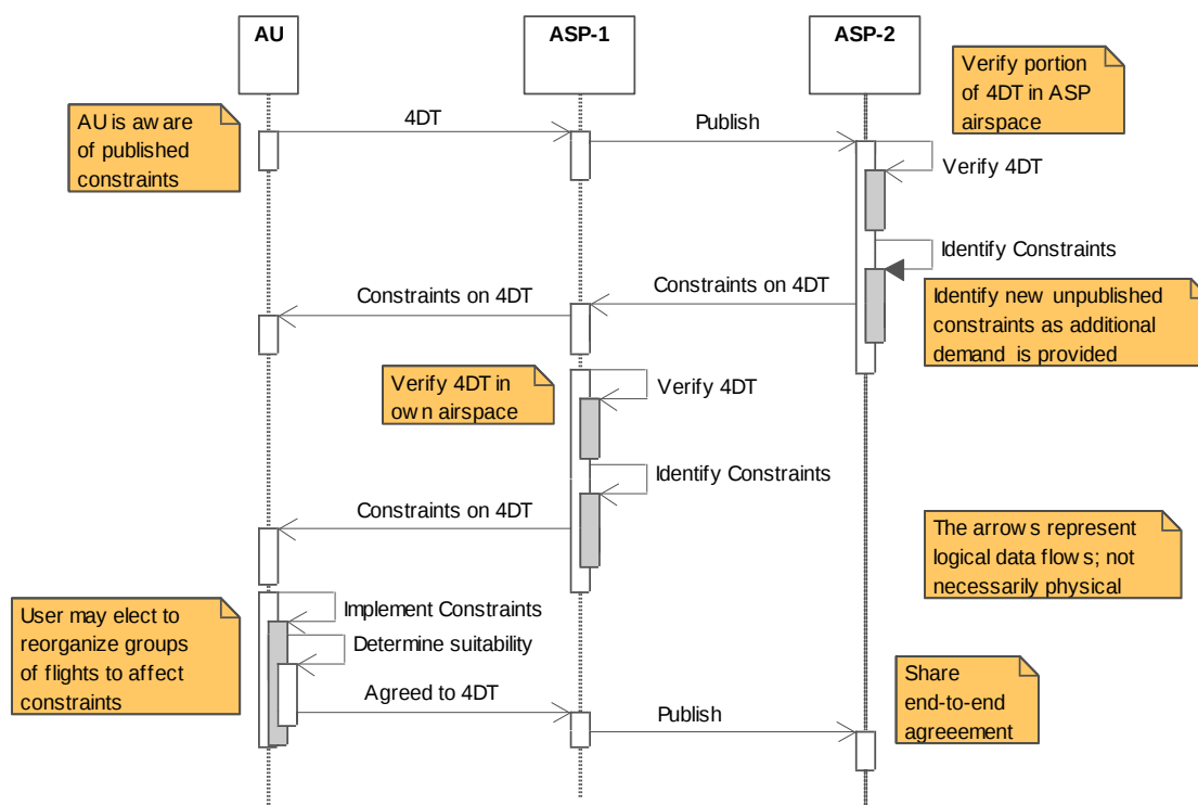
Figure C.6-2 Determining Agreed 4D trajectory using constraints
