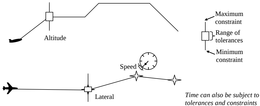
Figure D.2-3 Illustration of 4D tolerances and constraints
