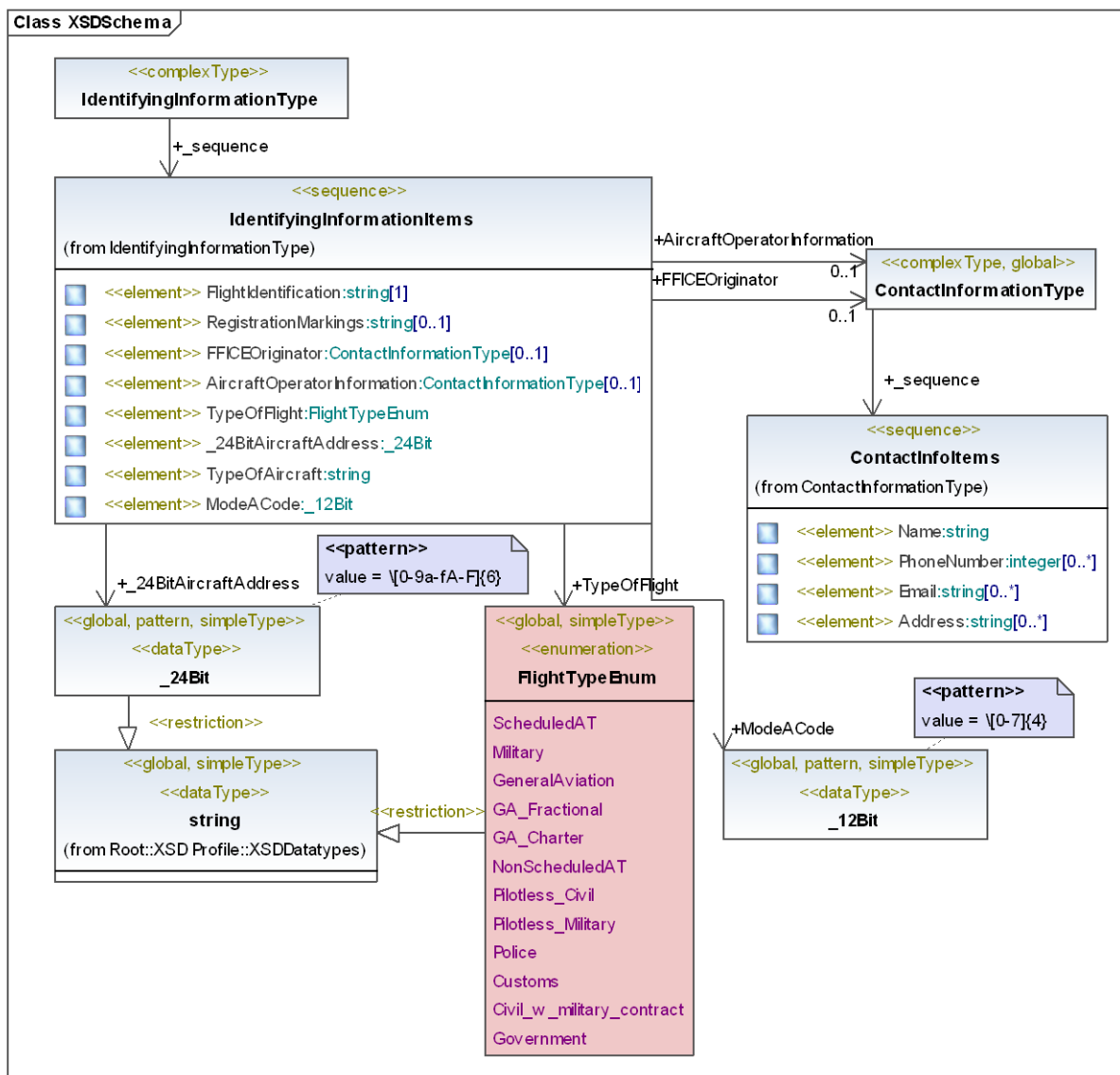
Figure G.2-5 Identifying Information XML schema Diagram
