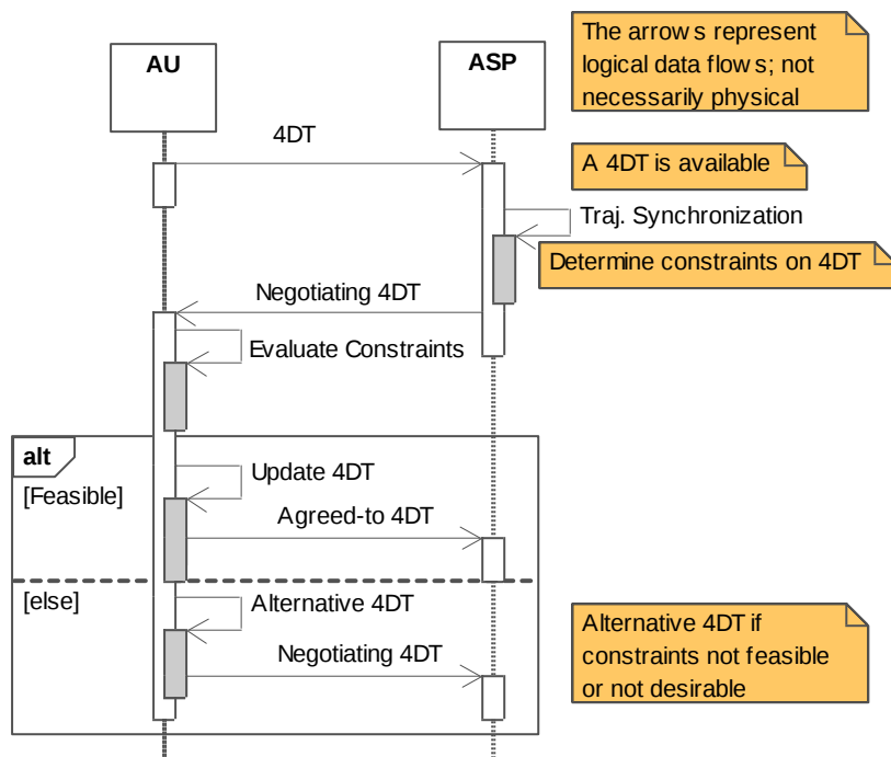
Figure C.6-7 Imposition of constraints on 4D trajectory for trajectory synchronization
