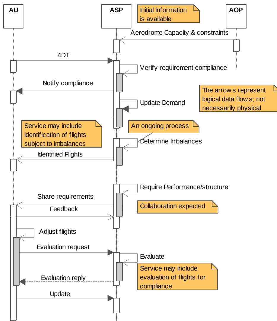
Figure C.5-1 Illustration of imposition of airspace structure or performance requirements to deal with expected imbalances
