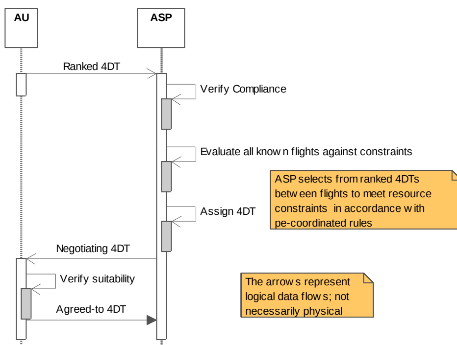
Figure C.6-5 Selection of ranked 4D trajectory
