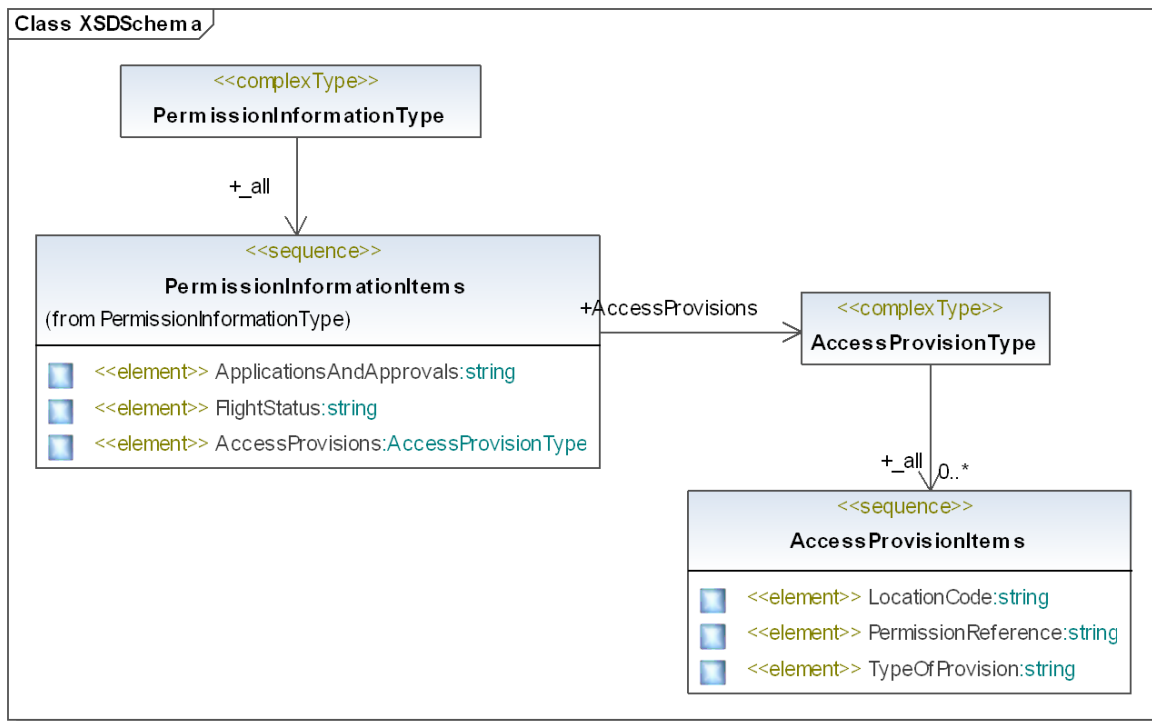
Figure G.2-7 Permission XML schema Diagram
