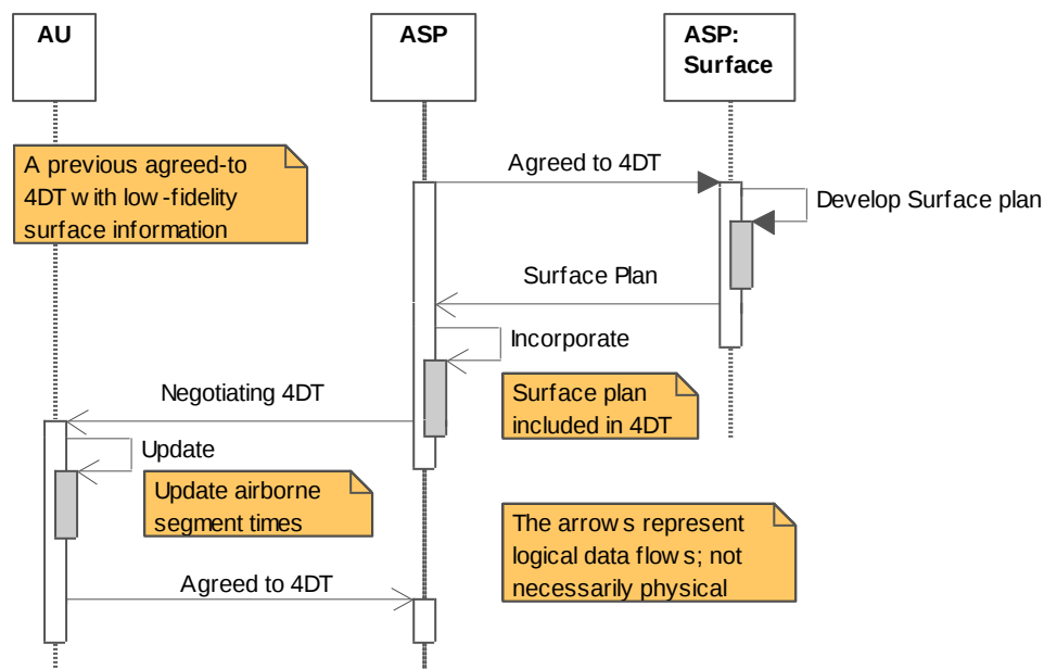
Figure C.6-6 Development of a surface plan on departure
