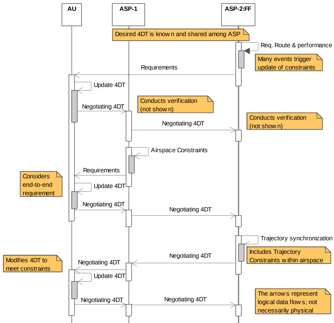
Figure C.7-2 Illustration of negotiation example in multi-ASP environment
