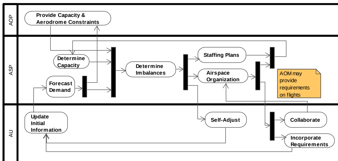
Figure C.3-1 Activity diagram for strategic planning
