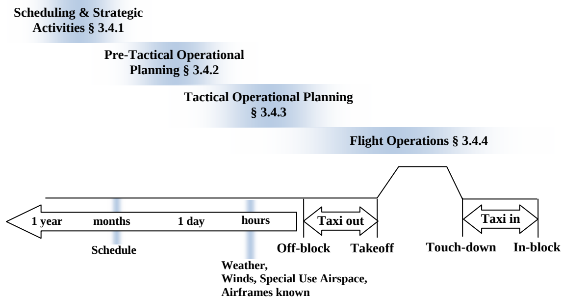
Figure 3.4-1 Timeline of information provision relative to events pertaining to a single flight. Referenced Sections detail FF-ICE activities in more detail.
