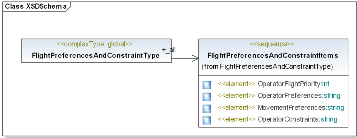
Figure G.2-8 Preferences XML schema Diagram
