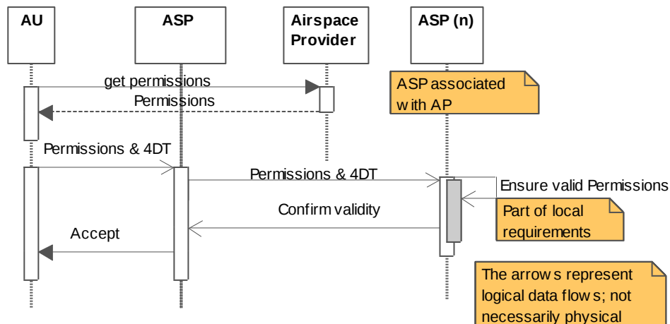
Figure C.4-1 Illustration of a candidate sequence for permission provision and verification
