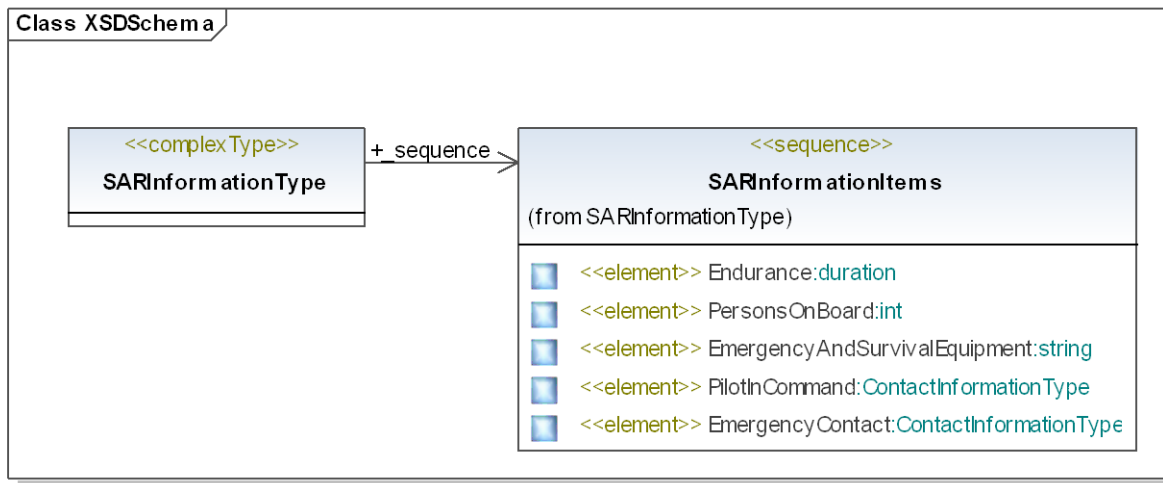
Figure G.2-9 SAR Information XML schema Diagram
