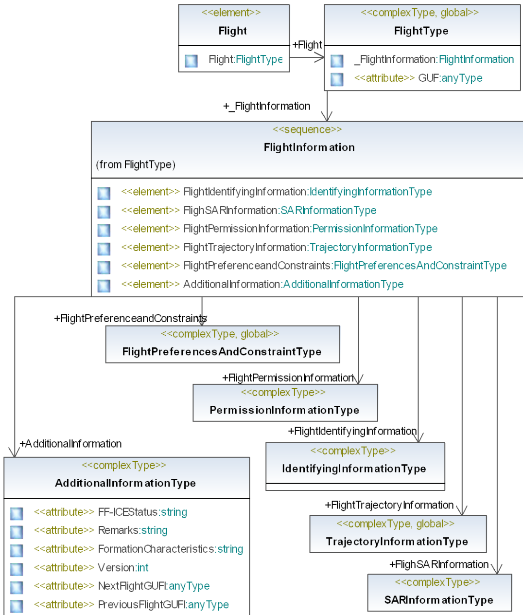
Figure G.2-1 Top Level Flight XML schema Diagram
