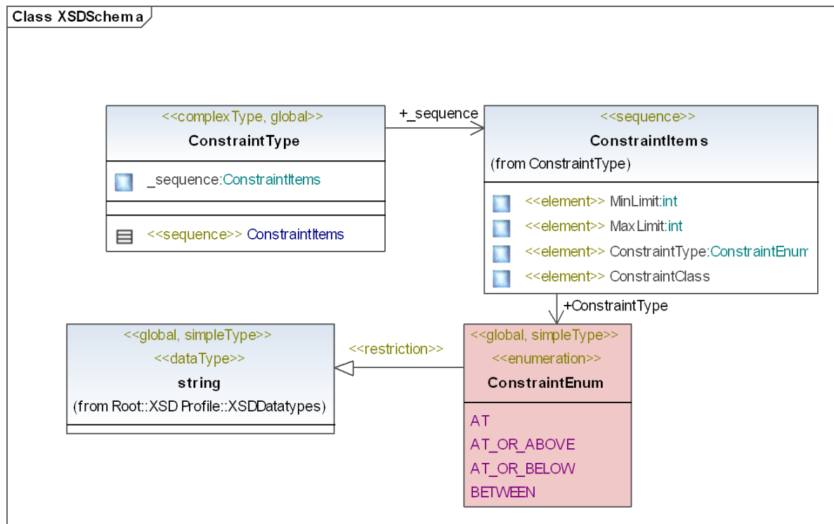
Figure G.2-4 Constraints XML schema Diagram
