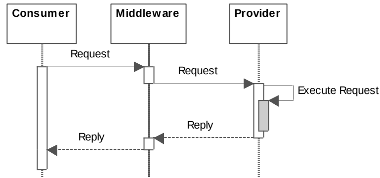
Figure H.1-5 Synchronous request/reply message pattern
