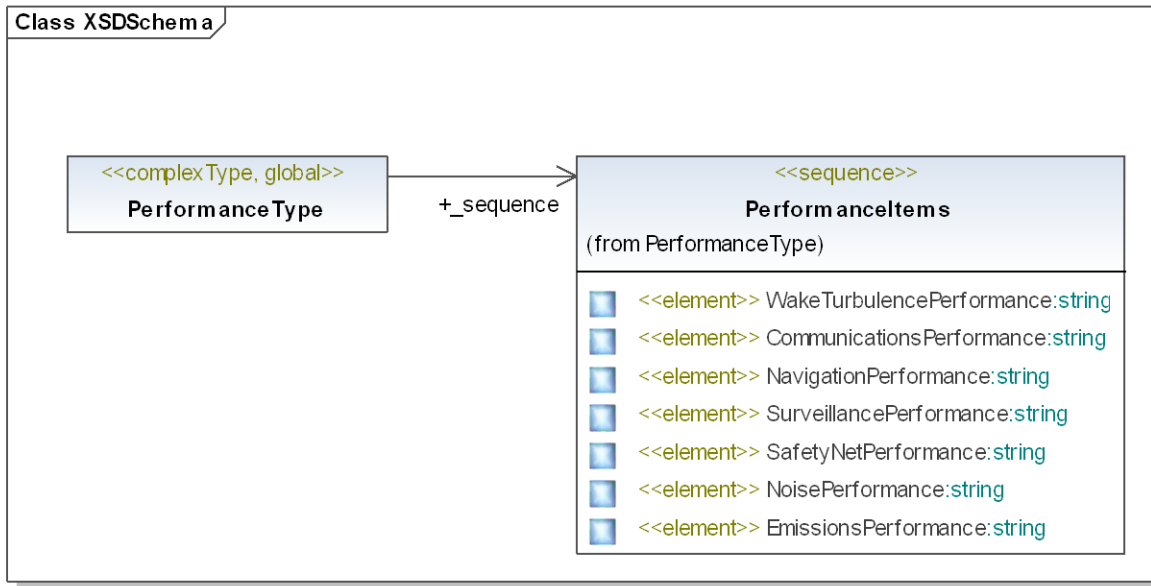
Figure G.2-6 Performance XML schema Diagram
