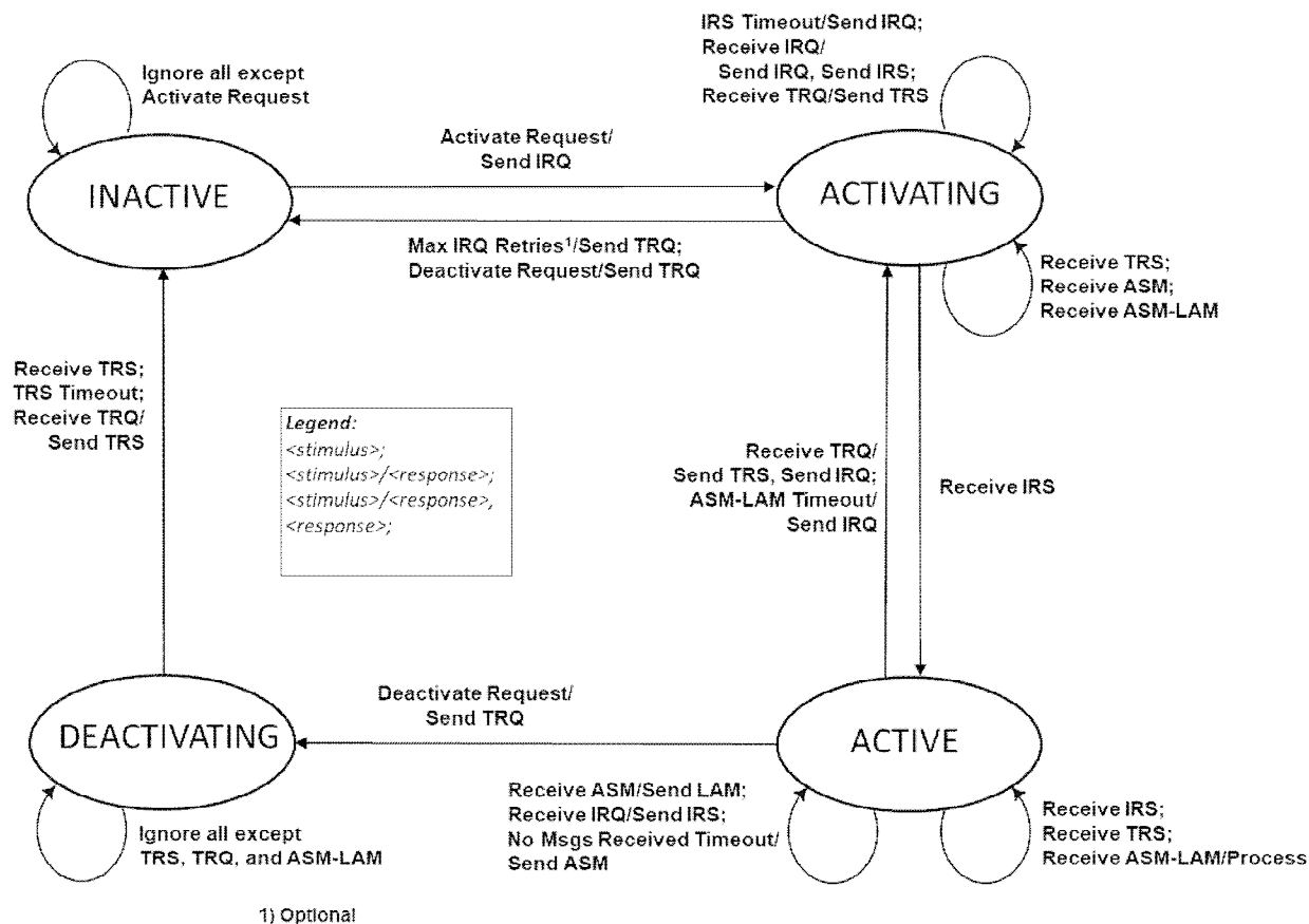
Figure 3-3. ERAM ARTCC/Non-US ACC Session State Diagram with Stimuli and Responses.
