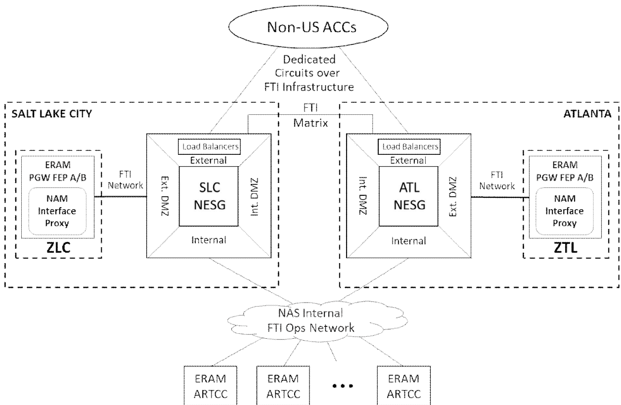
Figure 3-2. ERAM, Non-US ACC System Interface Connections.
