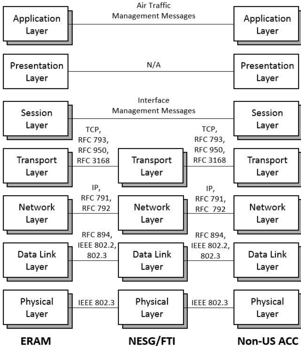
Figure 3-4. OSI Protocol Mapping for ERAM/Non-US ACC Systems
