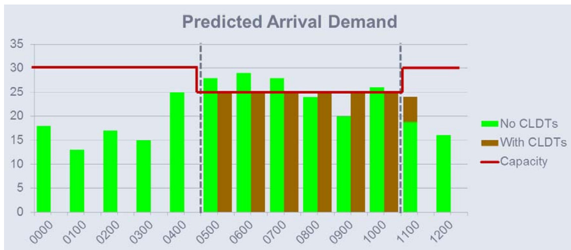
Figure 9: Modelled ATFM program
