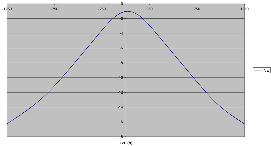
Figure 2.2 Logarithm (base 10) of TVE probability density defined by eq. (2.16)
