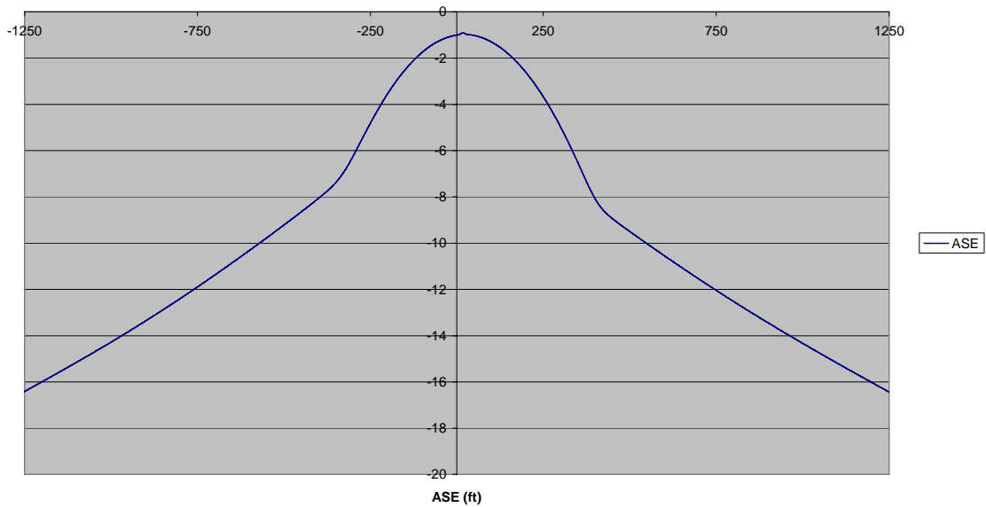
Figure A.2 Logarithm (base 10) of the overall ASE probability density for the AFI RVSM aircraft population
