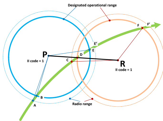
Figure 5 – SSR Mode S interrogator clustering (interrogators with same II code)
