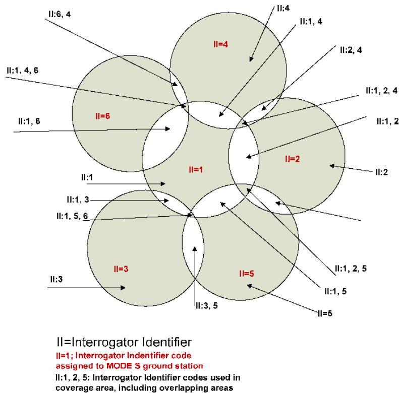
Figure 8 – Example of II code assignments
