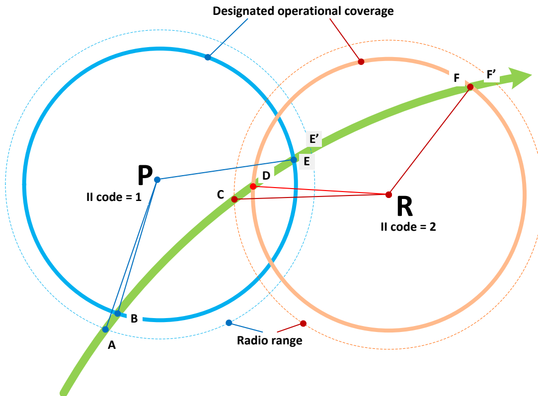
Figure 4 Process for II code acquisition and lock-out
