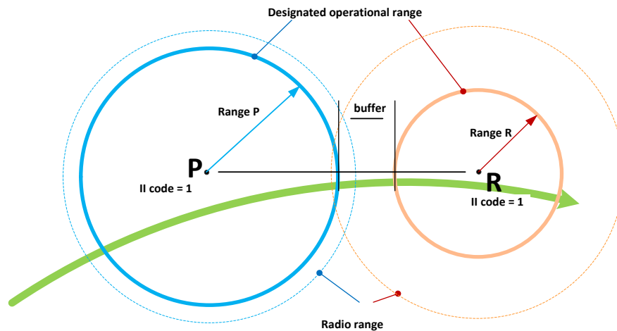
Figure 9 – Minimum separation distance between interrogators having the same II code
