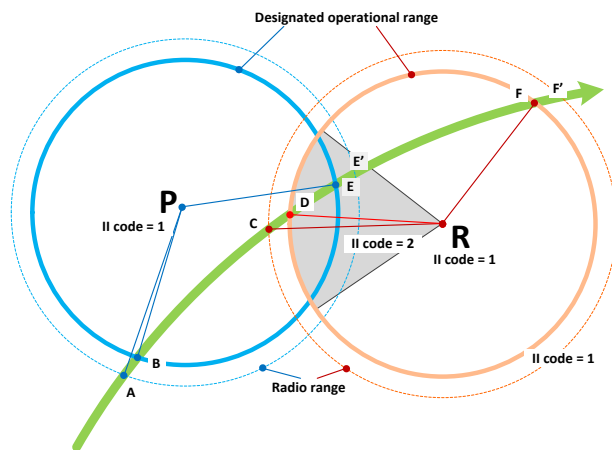
Figure 6 – Sectorized use of II codes
