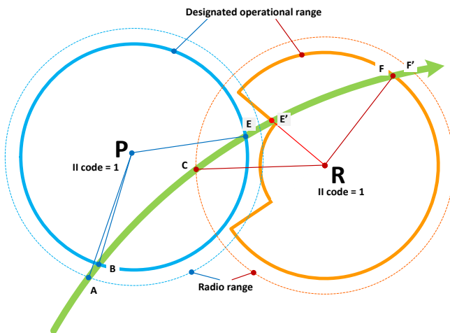
Figure 7 – Sectorized maximum range
