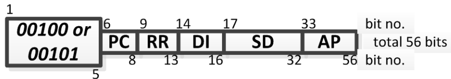
Figure 3A Uplink Format 4 and 5
