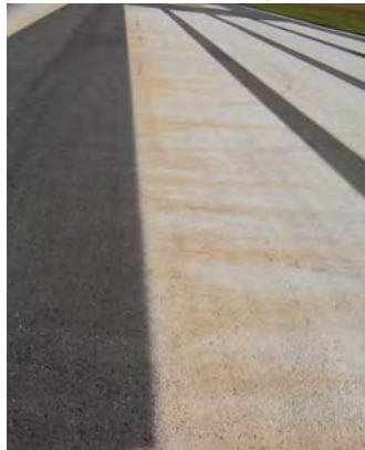
FIGURE 4-23. STAINED LEADING EDGE OF MARKING FROM IRON CONTAMINANTS.
