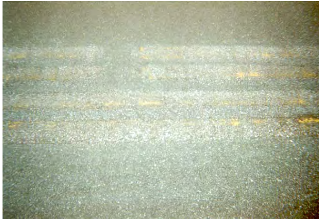
FIGURE 5-8. MINIMAL GRINDER SCARS ON ASPHALT AFTER REMOVING 90 PERCENT.
