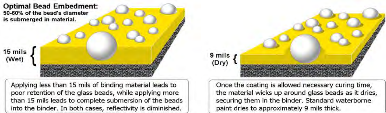
FIGURE 3-12. GLASS BEAD EMBEDMENT IN BOTH WET AND DRY PAINT FILM.
