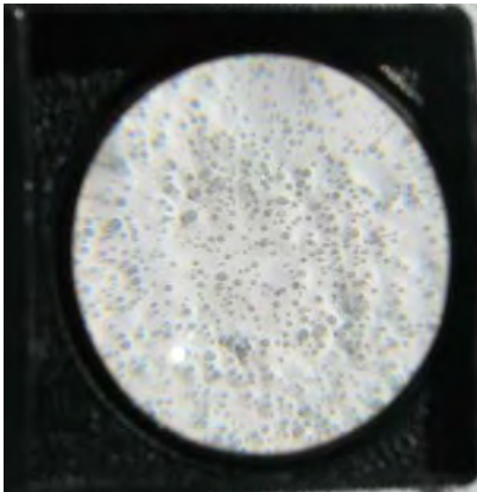
FIGURE 3-4. POOR TYPE I BEAD DISTRIBUTION; READINGS AVERAGED ONLY 135 mcd/m 2 /lux.
