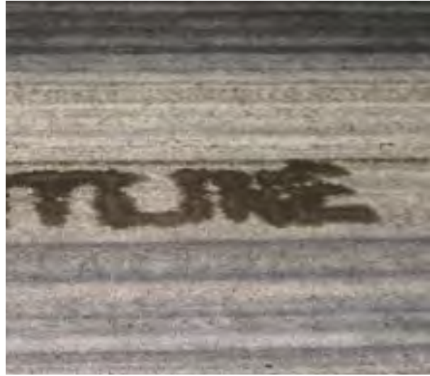
FIGURE 4-31. RUST REMOVER DAMAGED GLASS BEADS, MAKING THEM INEFFECTIVE.
