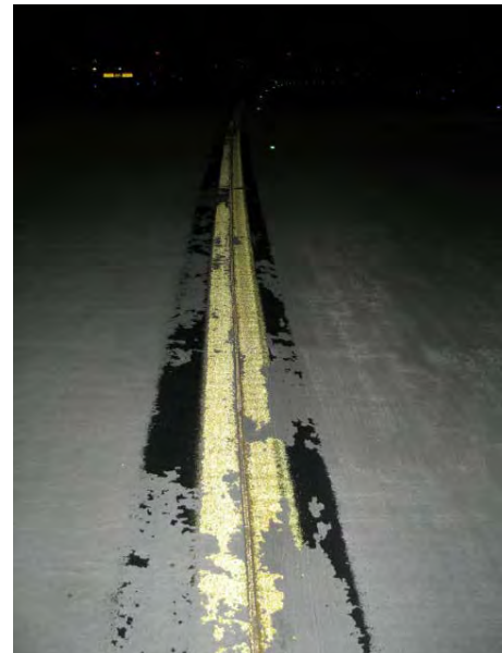
FIGURE 4-8. EXAMPLE OF POOR REMOVAL OF CURING COMPOUND.
