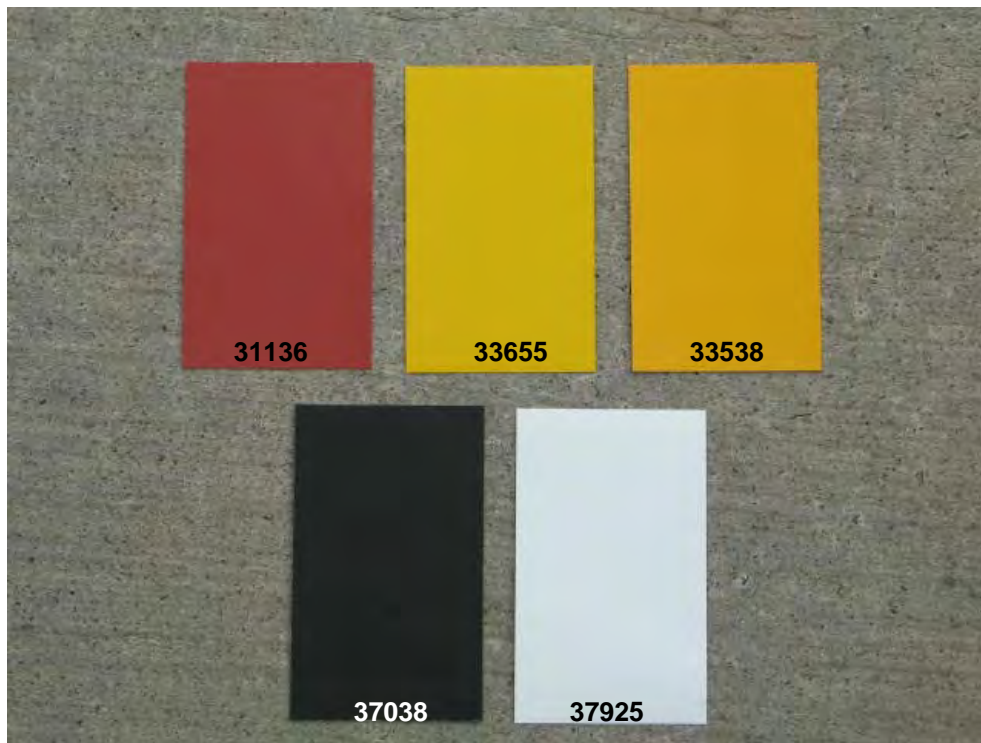
FIGURE 7-11. FEDERAL STANDARD 595B COLORS FOR AIRFIELD MARKINGS
