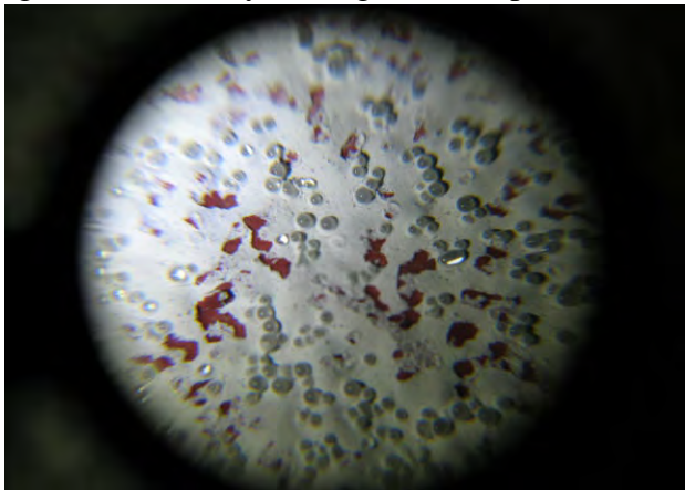
FIGURE 6-66. USE MAGNIFYING GLASS TO DETECT COATING PROBLEMS.
