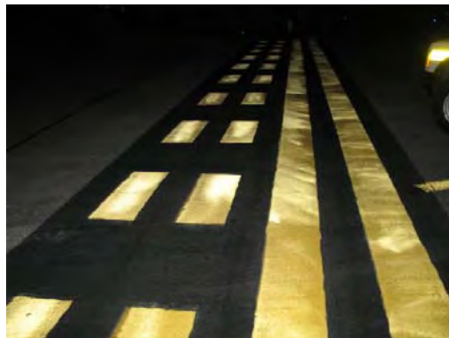
FIGURE 6-34. NEW HOLDING POSITION MARKING WHERE BEADS WERE HAND-THROWN.
