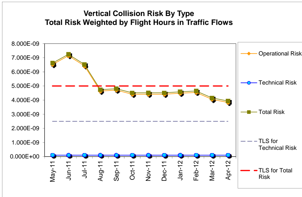
Figure 3. Vertical Collision Risk for Pacific RVSM Airspace
