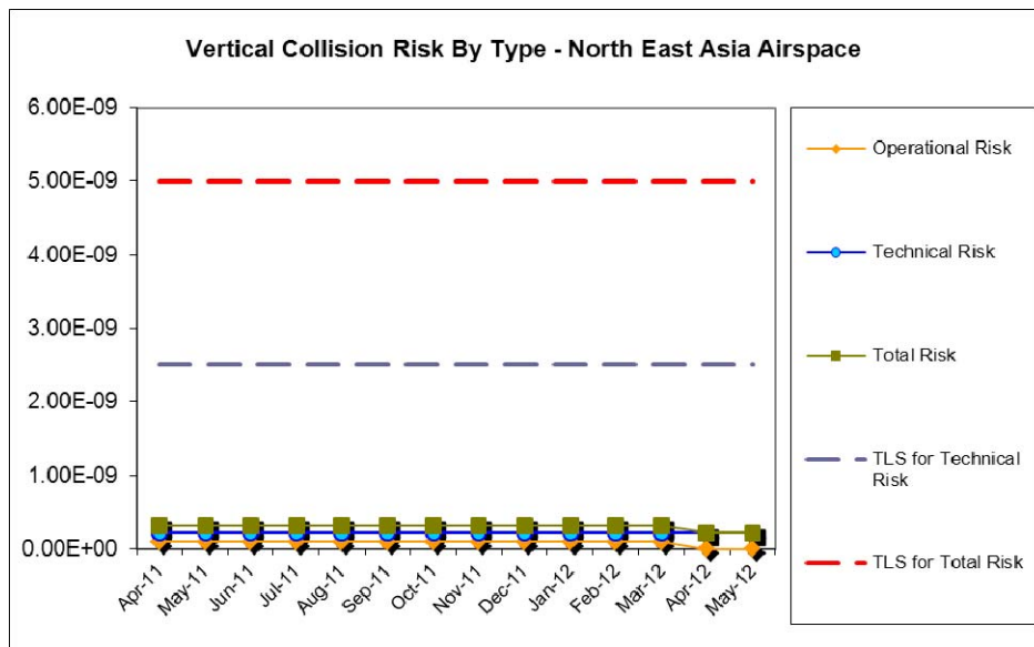
Figure 4. Vertical Collision Risk for North East Asia RVSM Airspace
