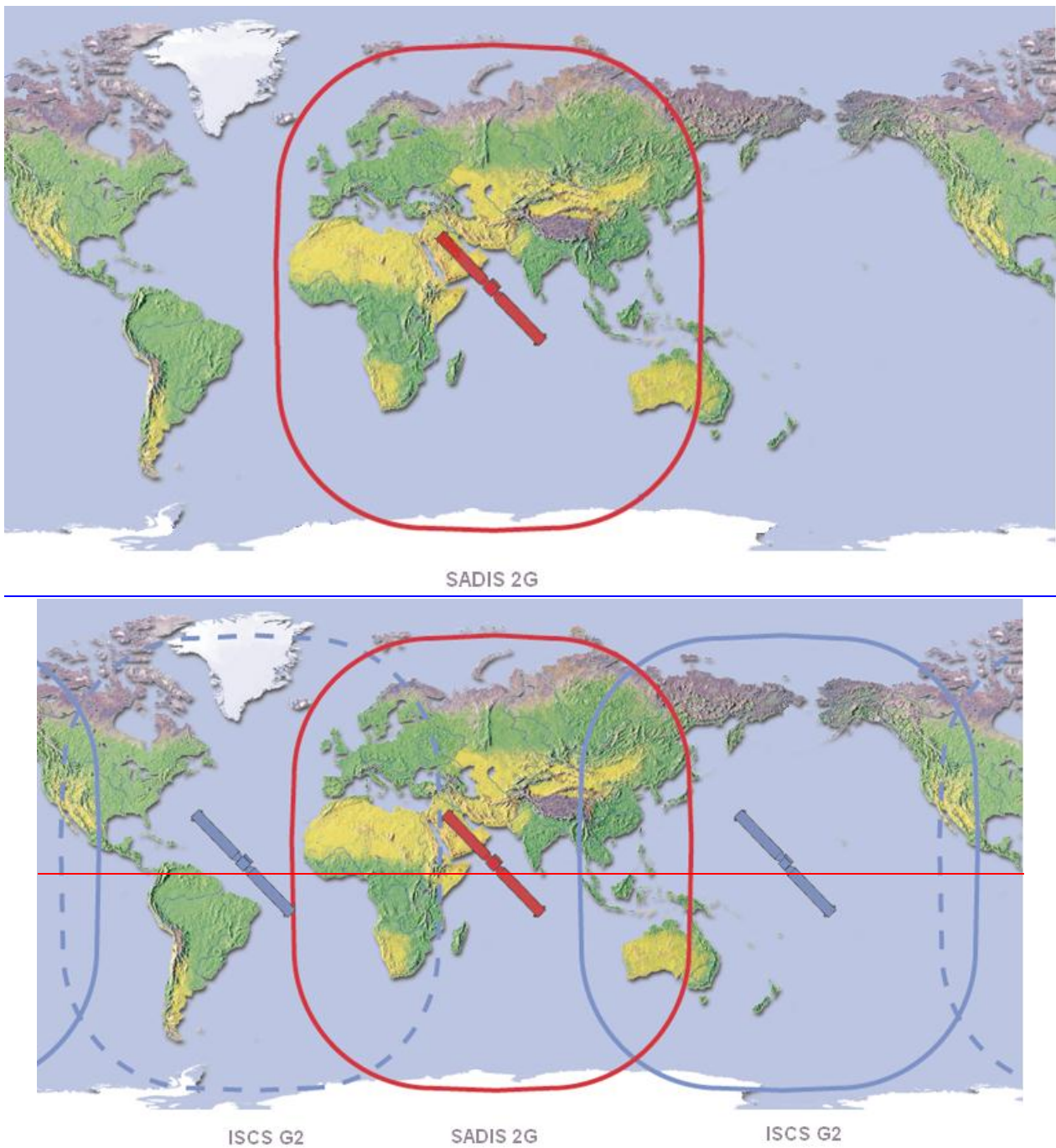
Figure 1: Schematic of ISCS G2 and SADIS 2G satellite footprints. Reception signal strengths, particularly at the edges of the footprints, are not so simply or sharply defined. Consult SADIS and ISCS guidance documents for detailed information.
