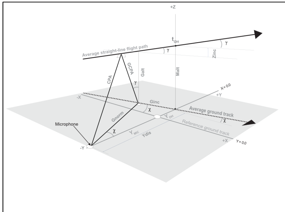
Figure 4-32. Detailed CPA geometry
