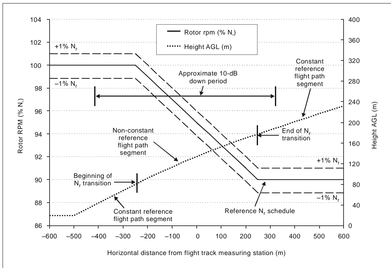
Figure 4-7. Example of a reference take-off flight path and rotor speed schedule (with \pm 1\% N_r limits) for a variable rotor speed helicopter
