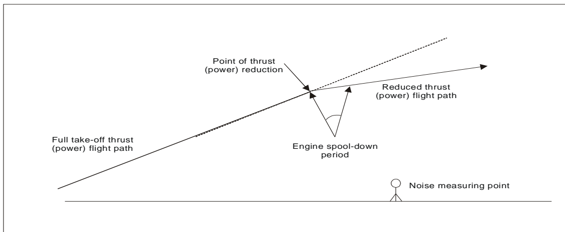
Figure 4-15. Take-off flight path over flyover measuring point with thrust (power) reduction
