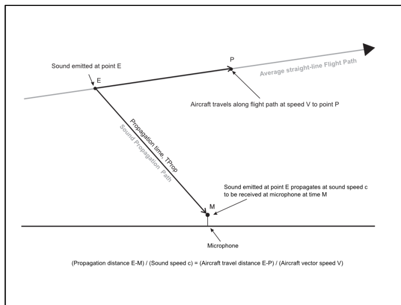
Figure 4-30. Aircraft position at time of sound emission
