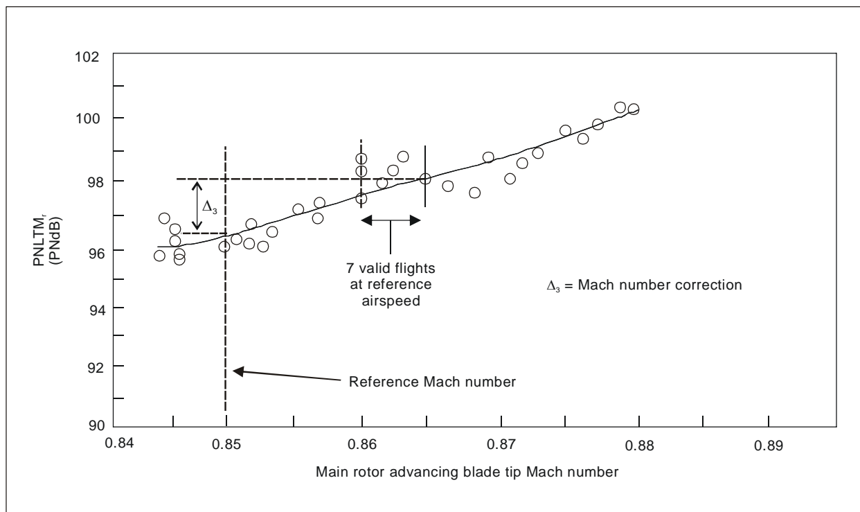
Figure 4-11. Example of source noise correlation using distributed test data
