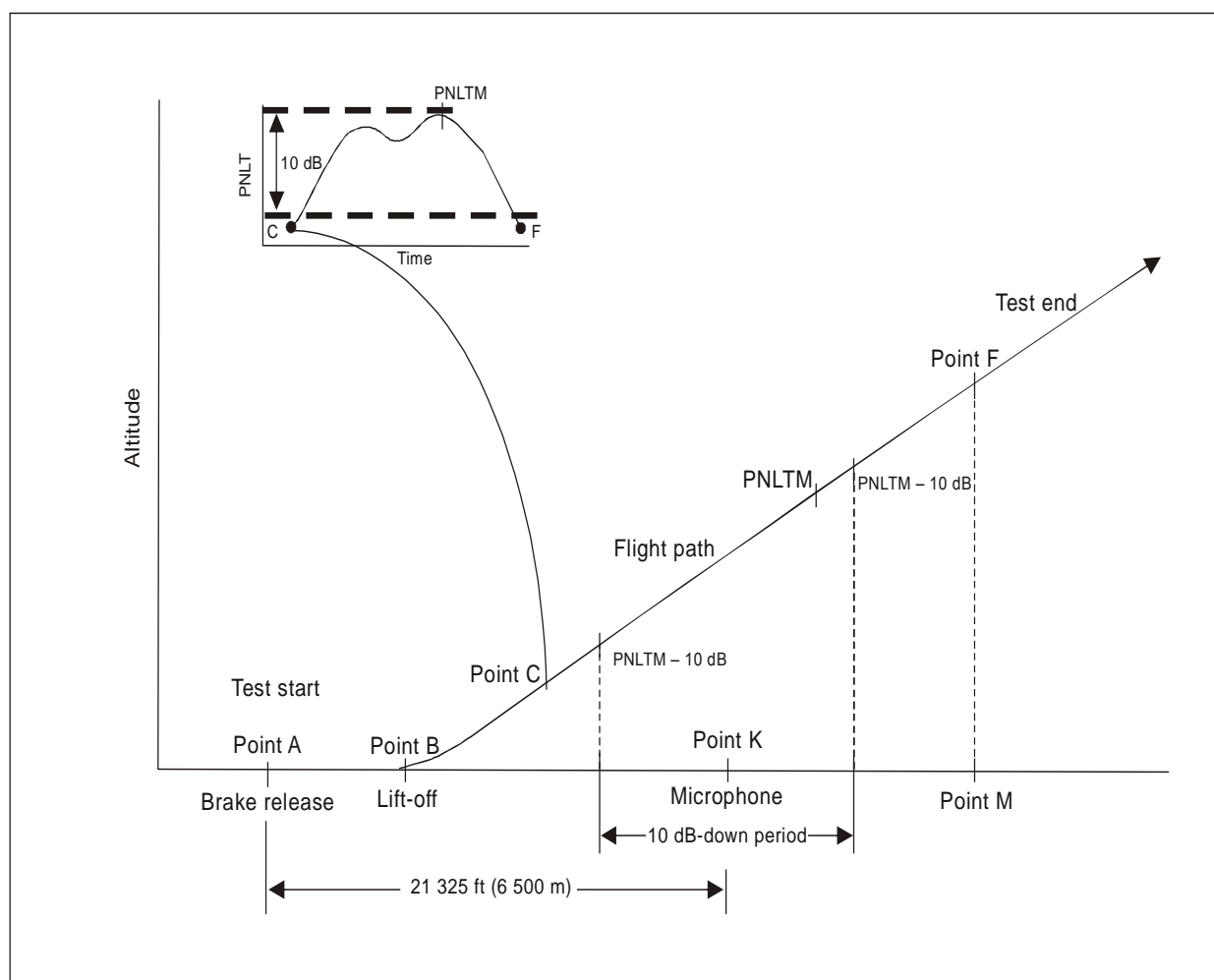
Figure 4-16. Normal full thrust (power) take-of
