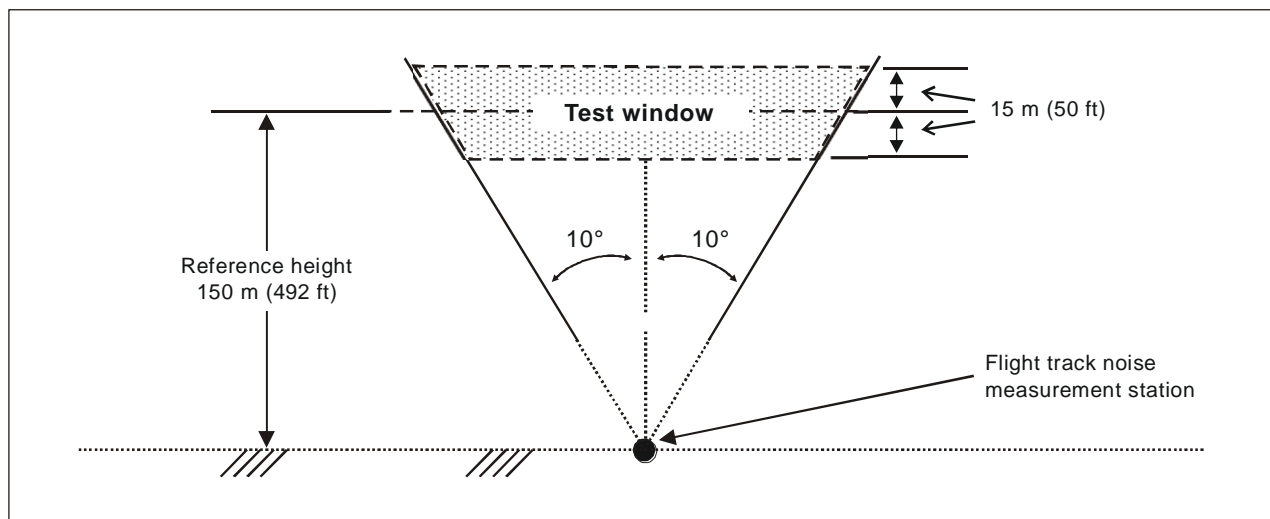
Figure 6-2. Flight boundaries for overflight test condition
