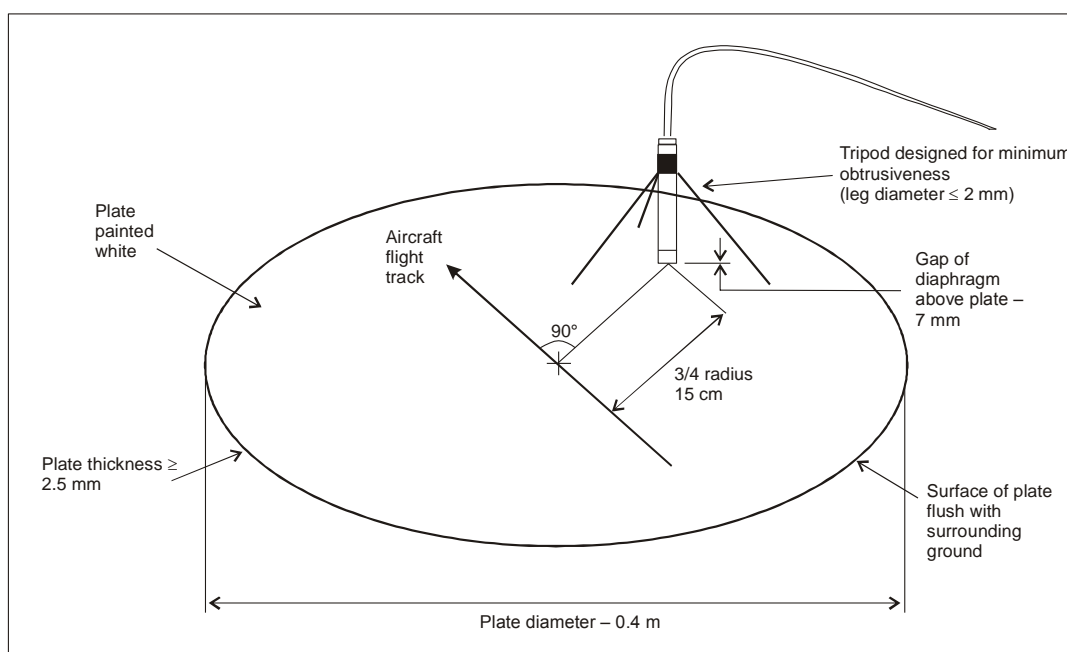
Figure 5-1. Configuration for one-half-inch inverted microphone
