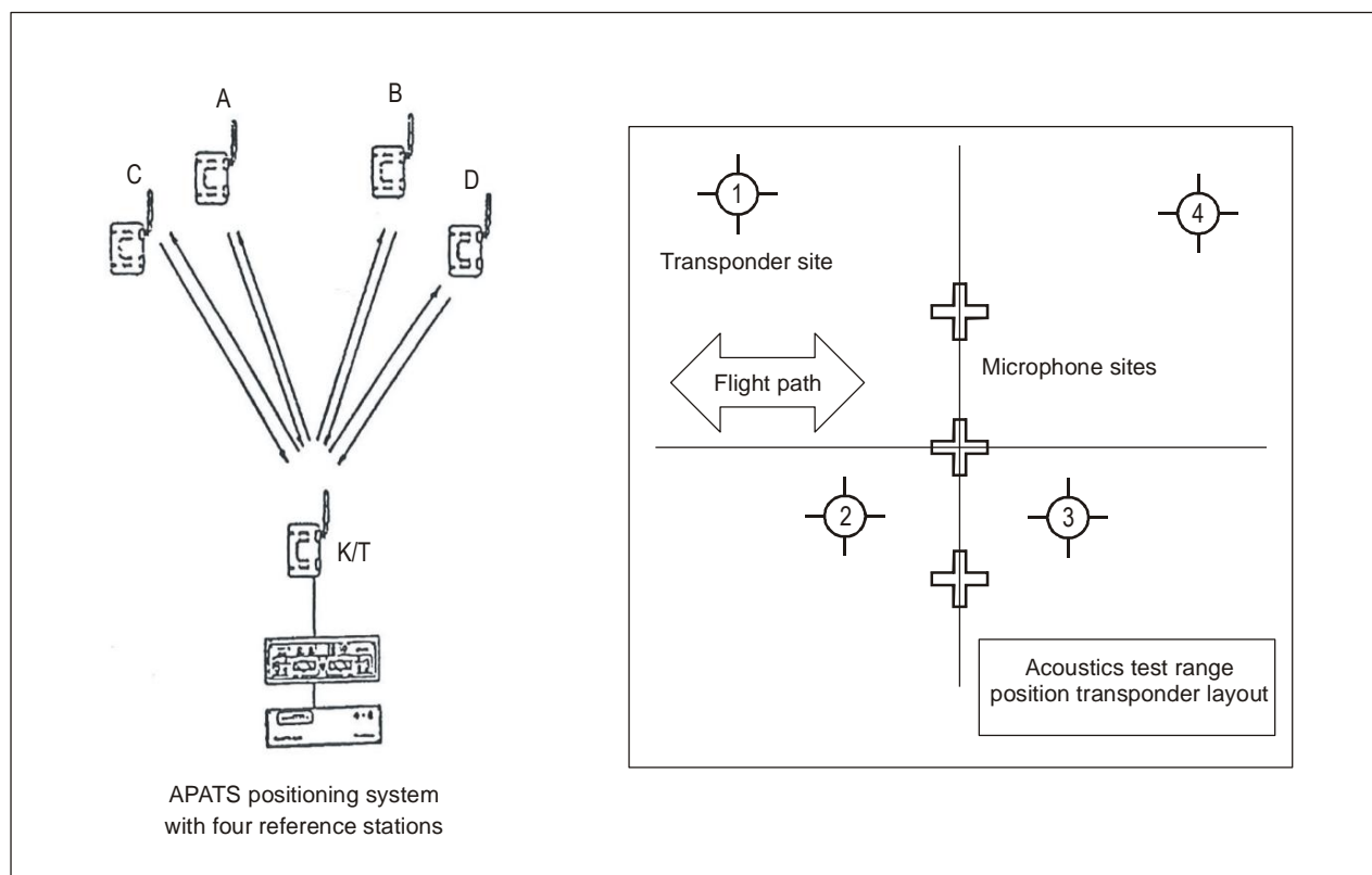
Figure 3-2. Example radar/microwave position tracking system
