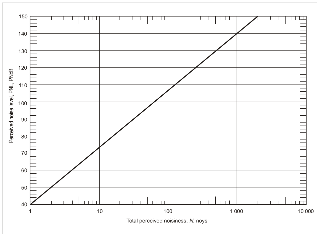
Figure 3-6. Perceived noise level as a function of total perceived noisiness
