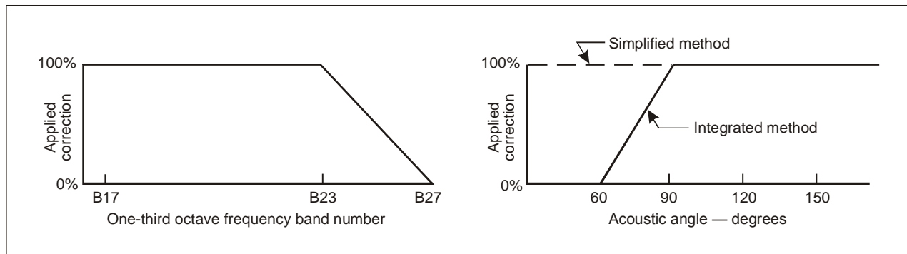
Figure 4-38. Criteria for jet source noise correction
