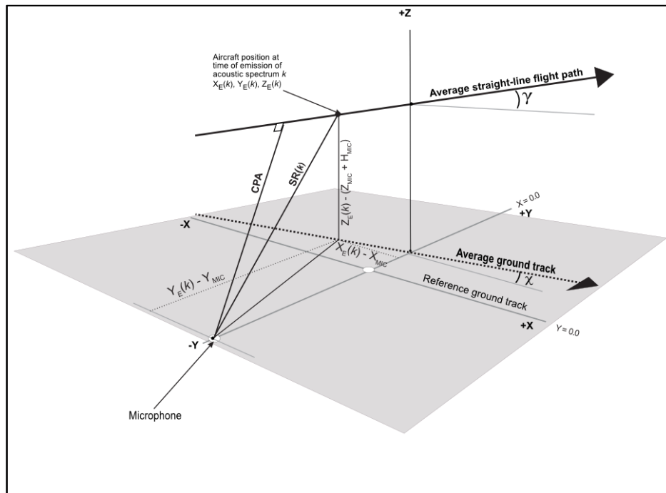
Figure 4-33. Sound propagation distance, SR(k)
