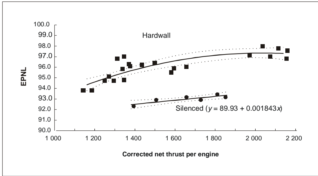
Figure 3-5. Regression curves for plots of EPNL against normalized thrust for hardwall and silenced conditions
