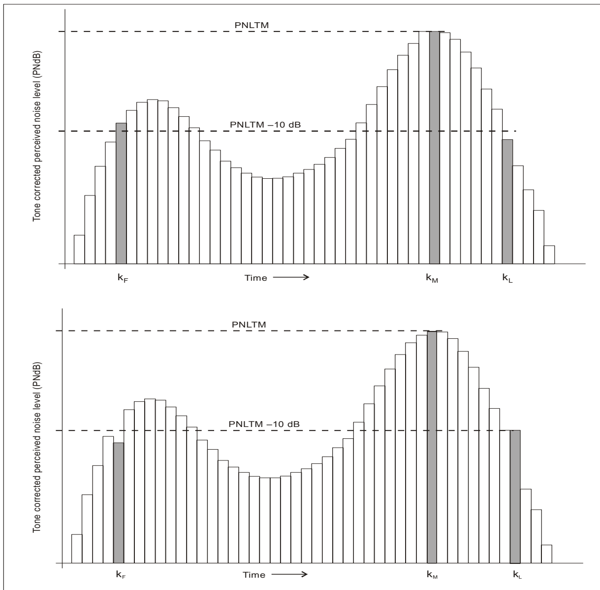
Figure 4-2. Illustrated example of identification of first and last 10 dB-down records
