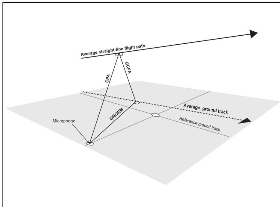
Figure 4-31. Basic CPA geometry
