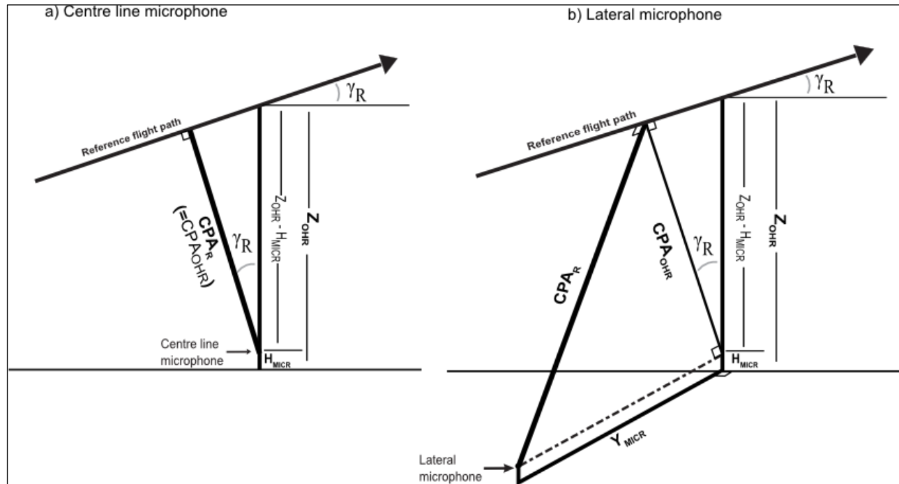
Figure 4-35. CPAR for centre line and lateral microphones
