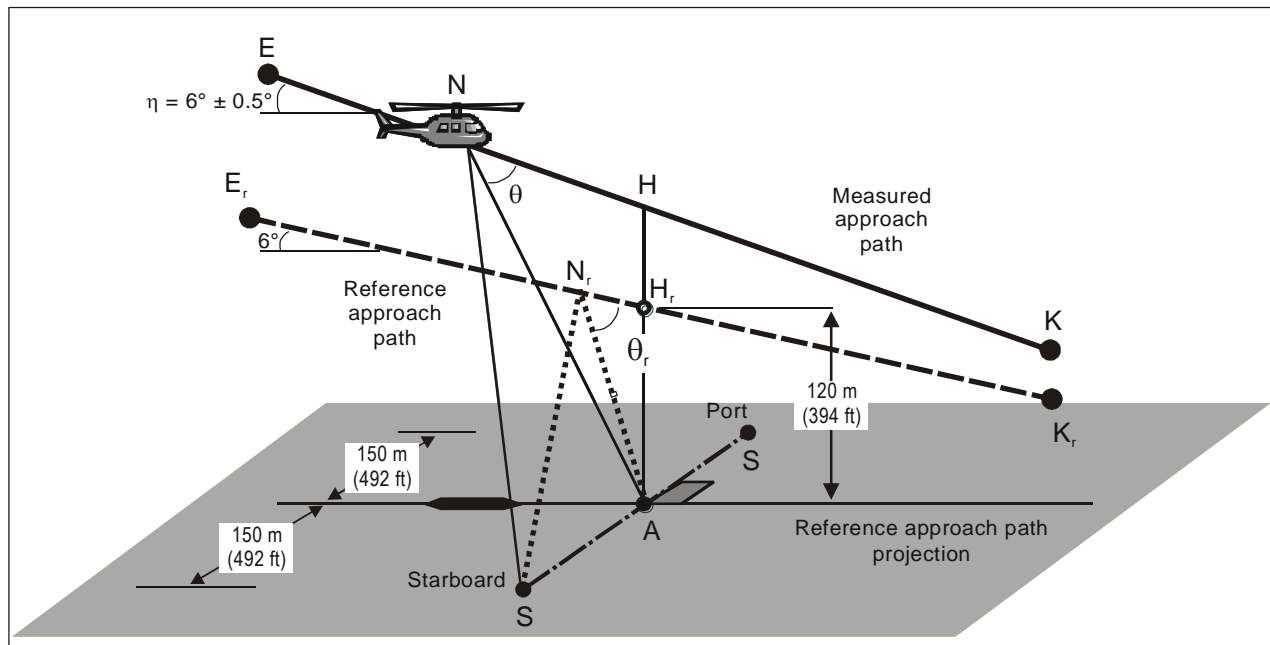
Figure 4-12. Comparison of measured and reference approach profiles
