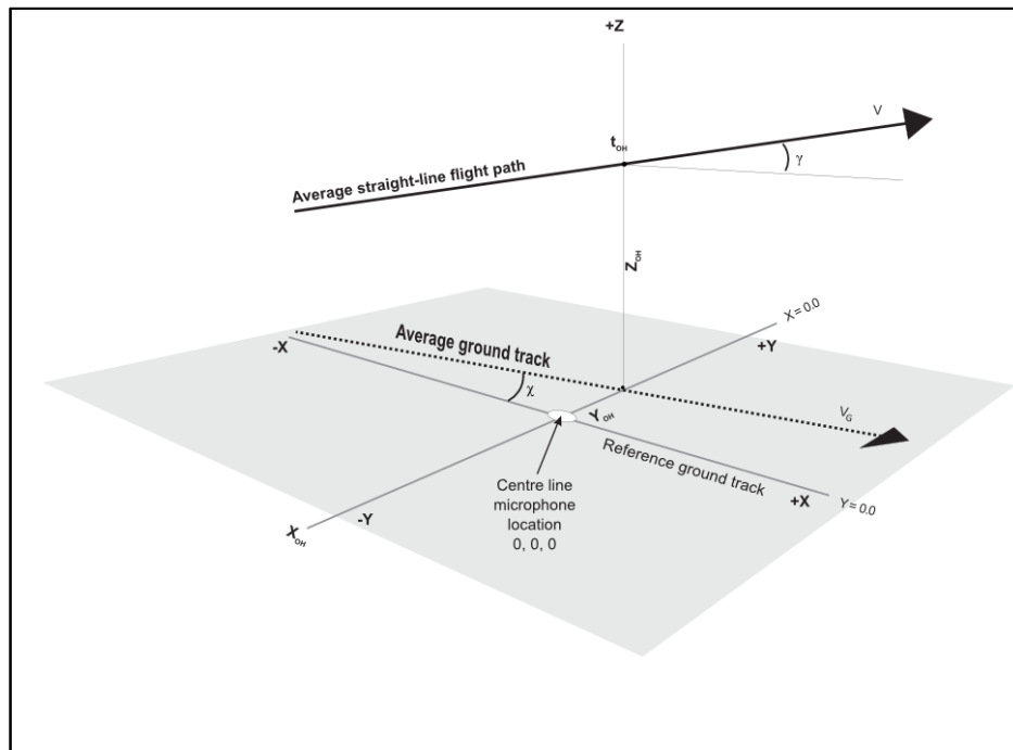
Figure 4-29. Single-point flight path descriptors
