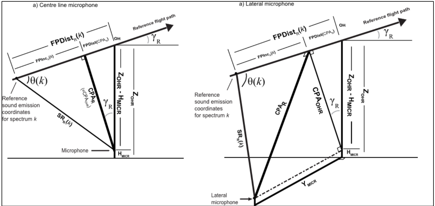
Figure 4-37. FPDist concept for centre line and lateral microphones
