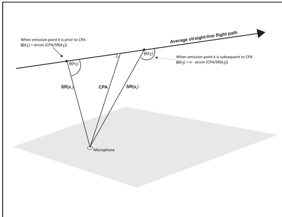
Figure 4-34. Acoustic emission angle, \theta
