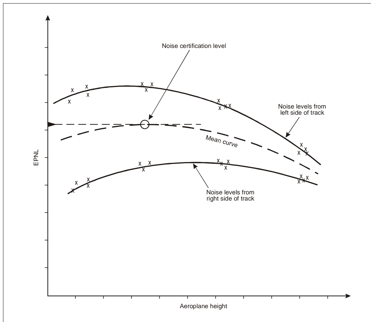
Figure 4-27. Typical lateral noise data plot for heavy propeller-driven aeroplanes
