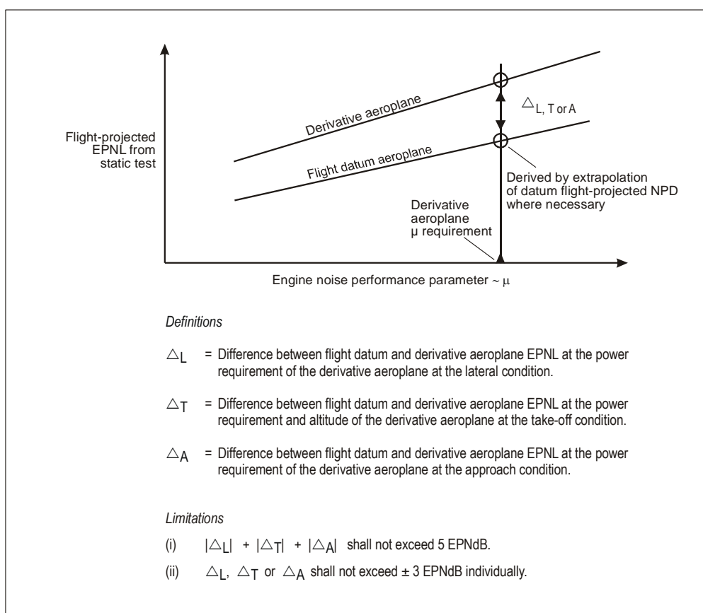
Figure 4-23. Limitation on use of static test when no validating flight data exist
