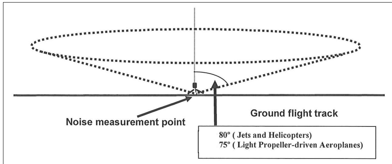
Figure 3-1. Obstruction-free cone defined from the base of the measurements microphone
