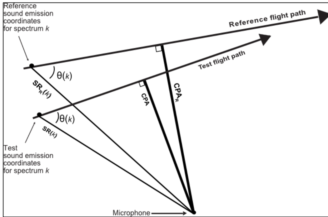
Figure 4-36. Determination of reference sound propagation distance, SRR(k)
