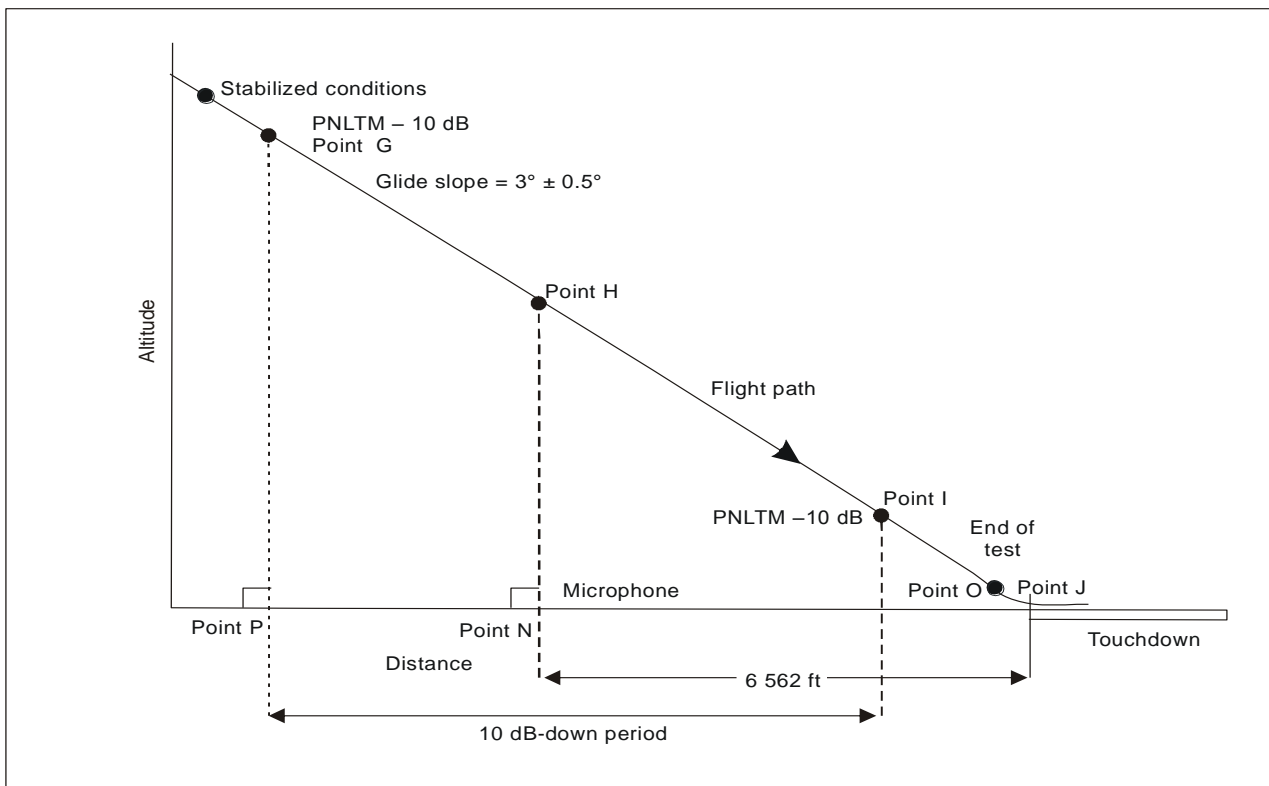
Figure 4-18. Approach with full landing
