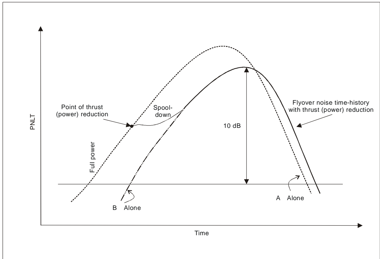
Figure 4-14. Take-off noise time history
