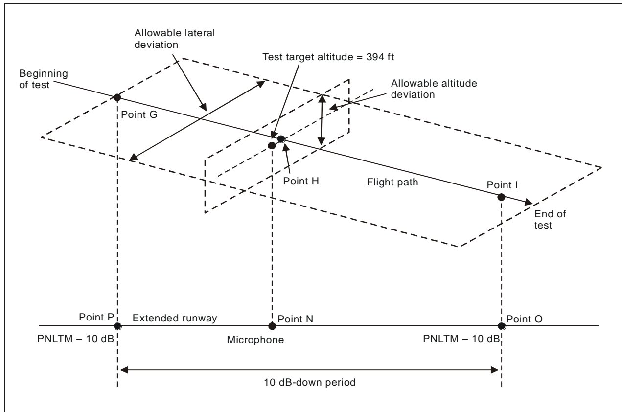
Figure 4-19. Approach flight path tolerances
