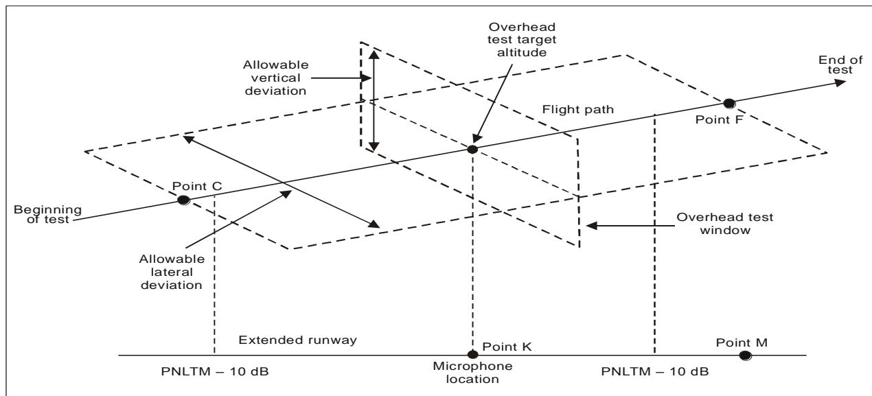
Figure 4-17. Take-off flight path tolerances
