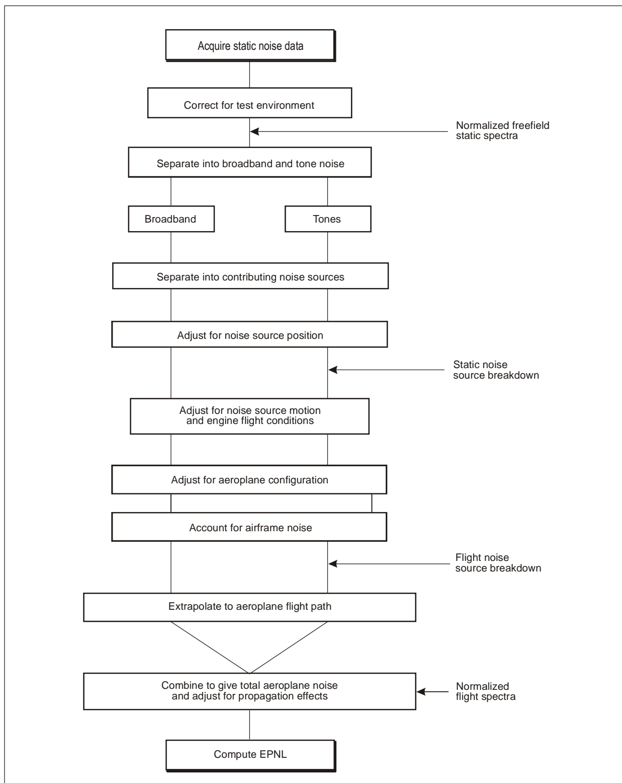
Figure 4-24. Generalized projection of static engine data to aeroplane flight conditions (Refer to 4.2.1.3)
