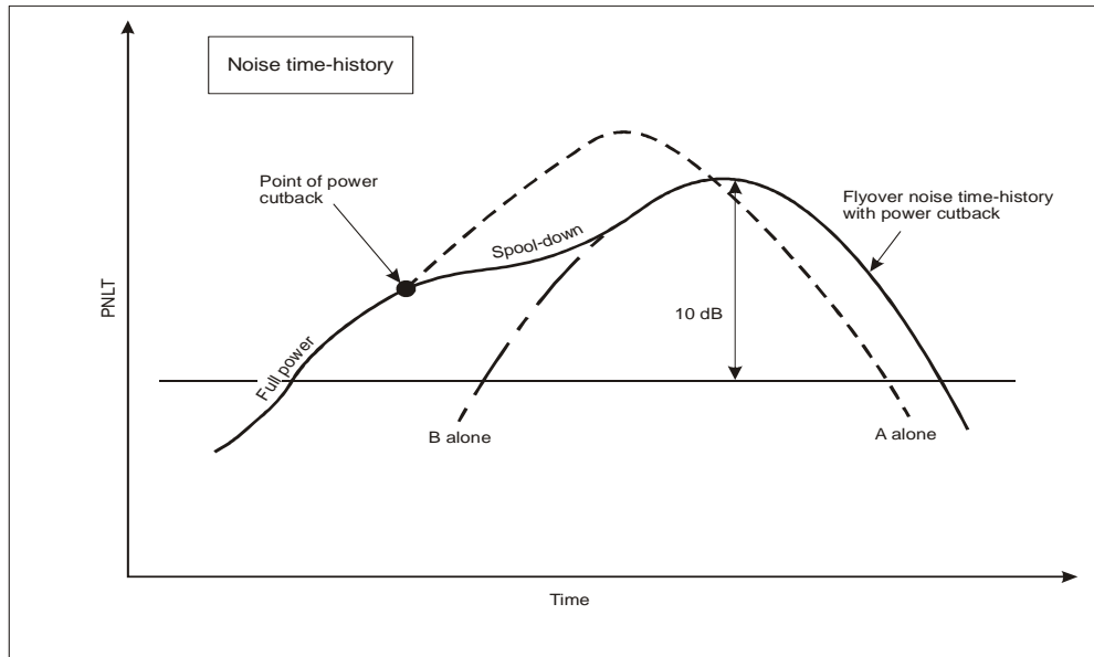
Figure 4-22 a). Computation of cutback take-off noise level from constant power tests
