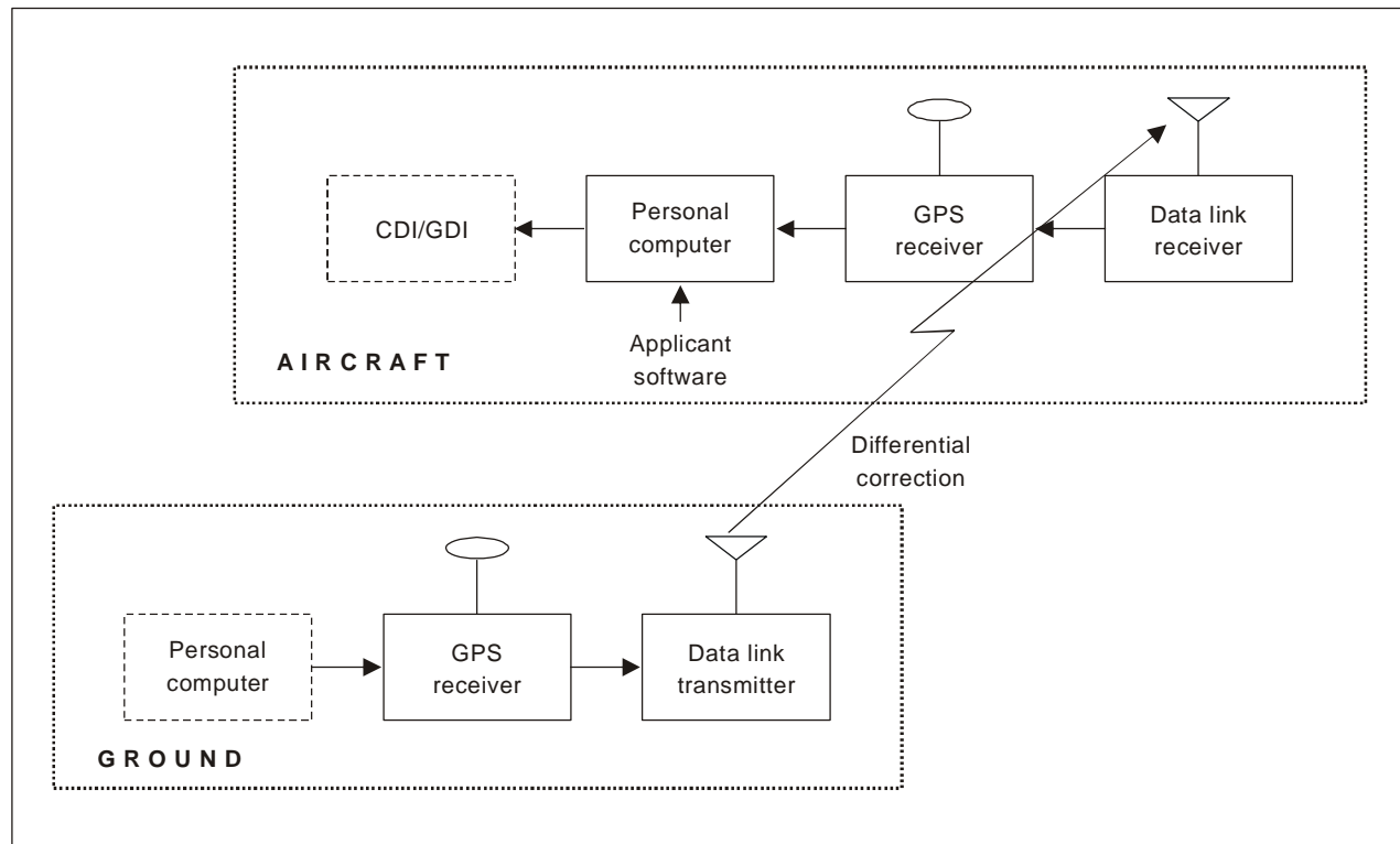
Figure 3-4. DGPS TSPI system basic architecture
