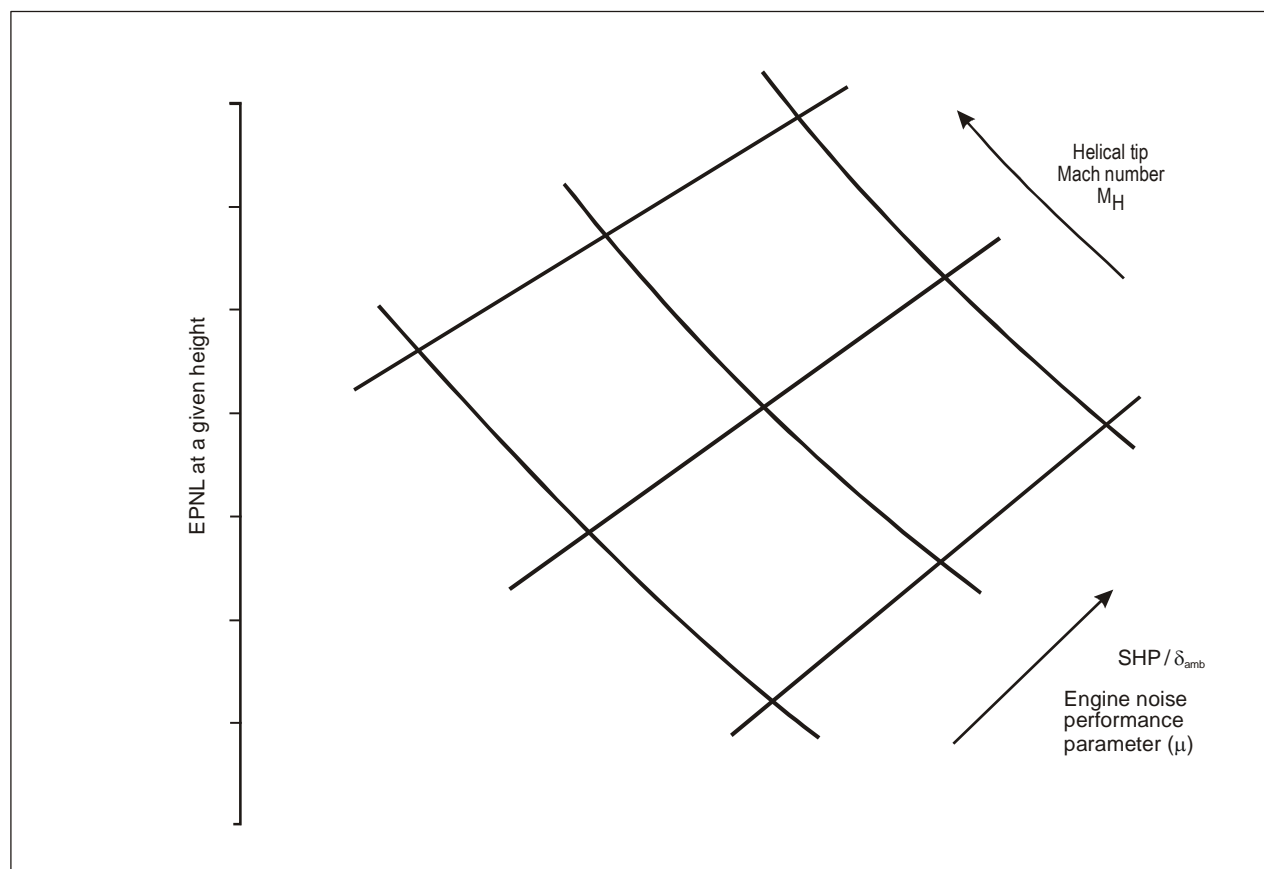
Figure 4-26. Form of noise-power-distance (NPD) plot for heavy propeller-driven aeroplanes
