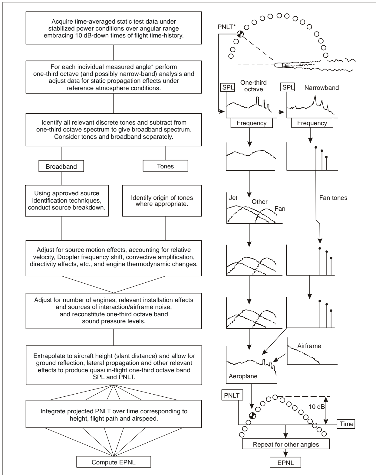
Figure 4-25. Example procedure for projection of static engine data to aeroplane flight conditions
