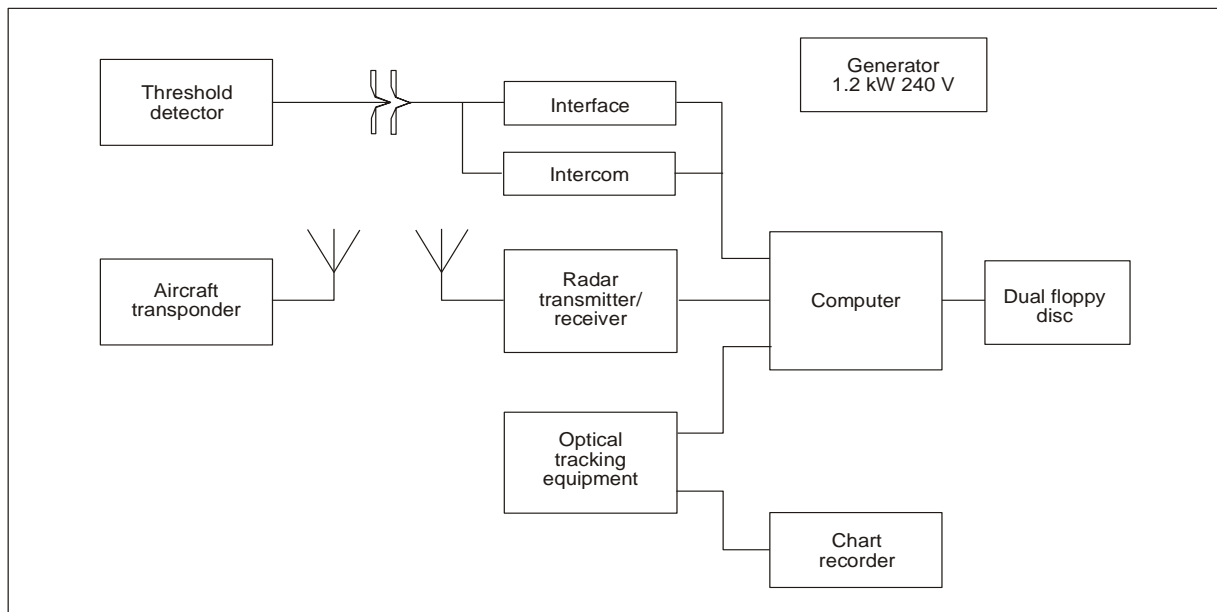
Figure 3-3. Radar/optical position tracking system
