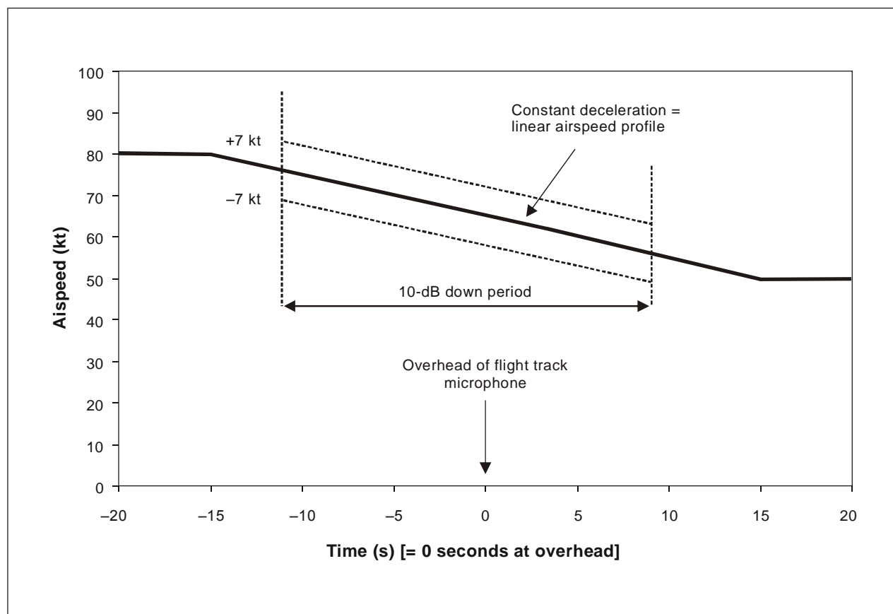
Figure 8-2. Example of a reference airspeed profile versus time for a constant deceleration from 80 kt to 50 kt at 1 kt/s
