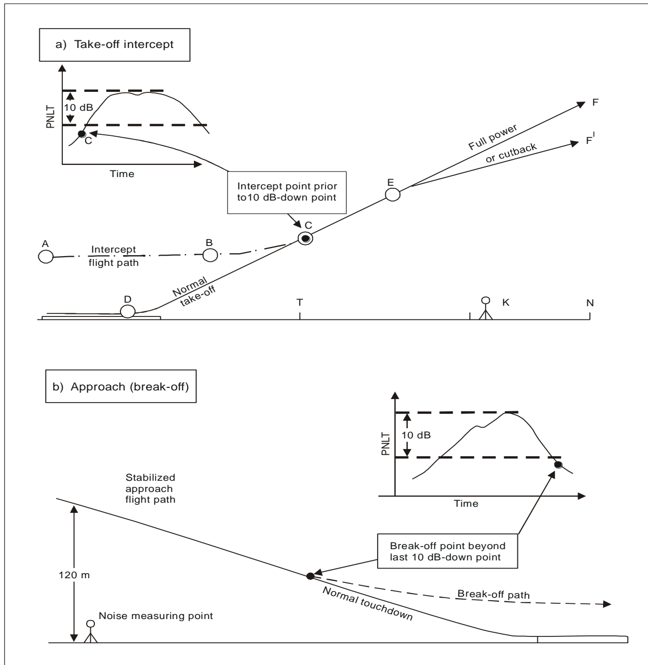
Figure 4-20. Flight path intercept procedures
