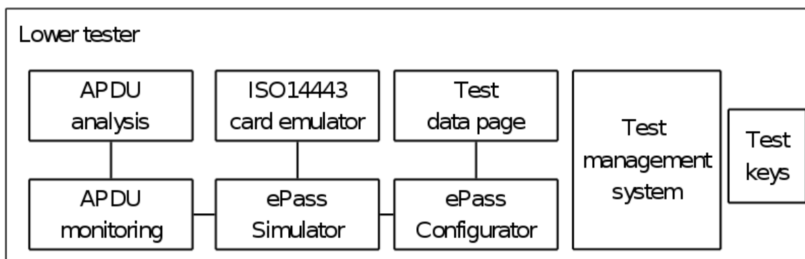
Figure 2: Functional components of the lower tester
